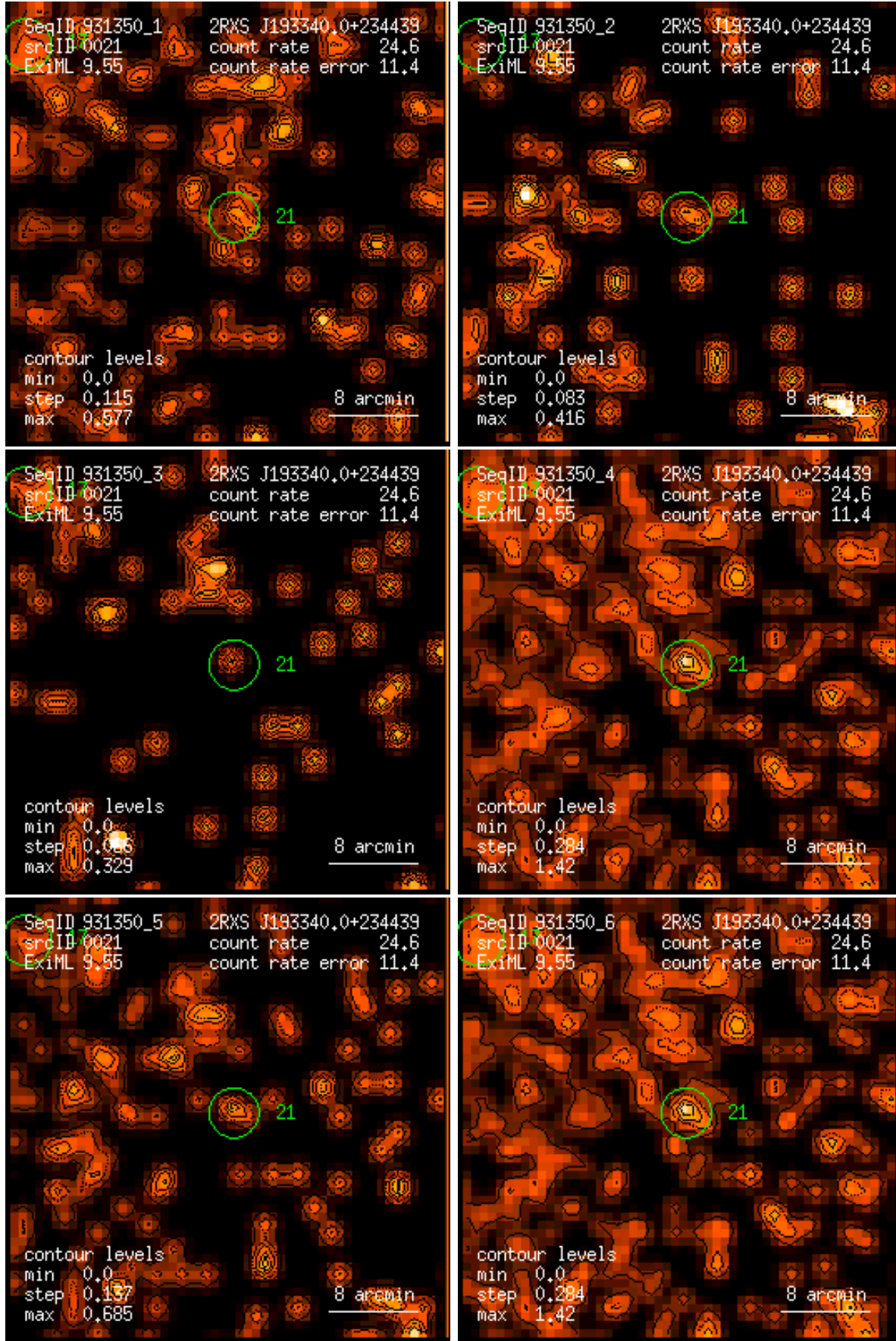
Figure 21: RASS 931350: detection 0021: band rate images, Gaussian filter: (1) PSPC channels 11 – 41, (2) 52 – 90, (3) 91 – 201, (4) 11 – 235, (5) 52 – 201, (6) 11 – 201. Broad band rates in counts/ks. Band rate contour levels in counts/ks/arcmin 2 .
