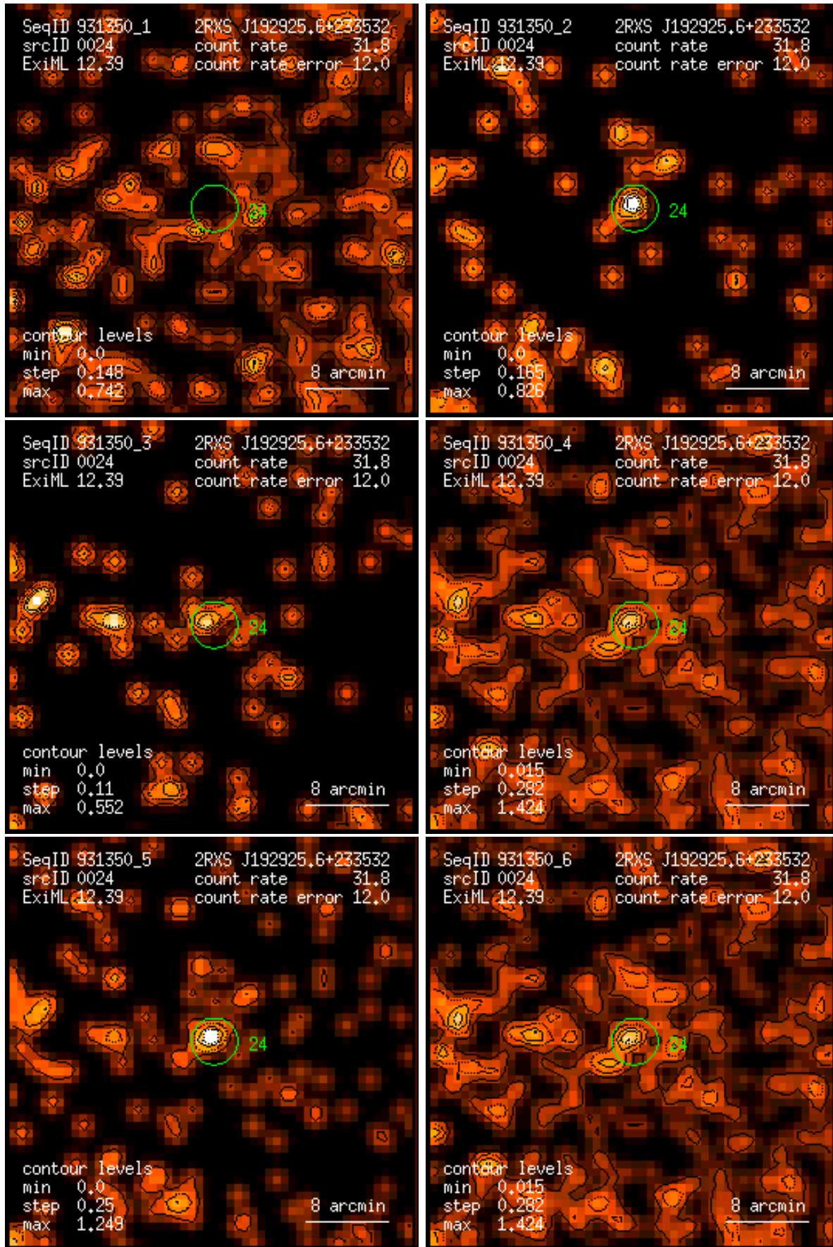
Figure 24: RASS 931350: detection 0024: band rate images, Gaussian filter: (1) PSPC channels 11 – 41, (2) 52 – 90, (3) 91 – 201, (4) 11 – 235, (5) 52 – 201, (6) 11 – 201. Broad band rates in counts/ks. Band rate contour levels in counts/ks/arcmin 2 .
