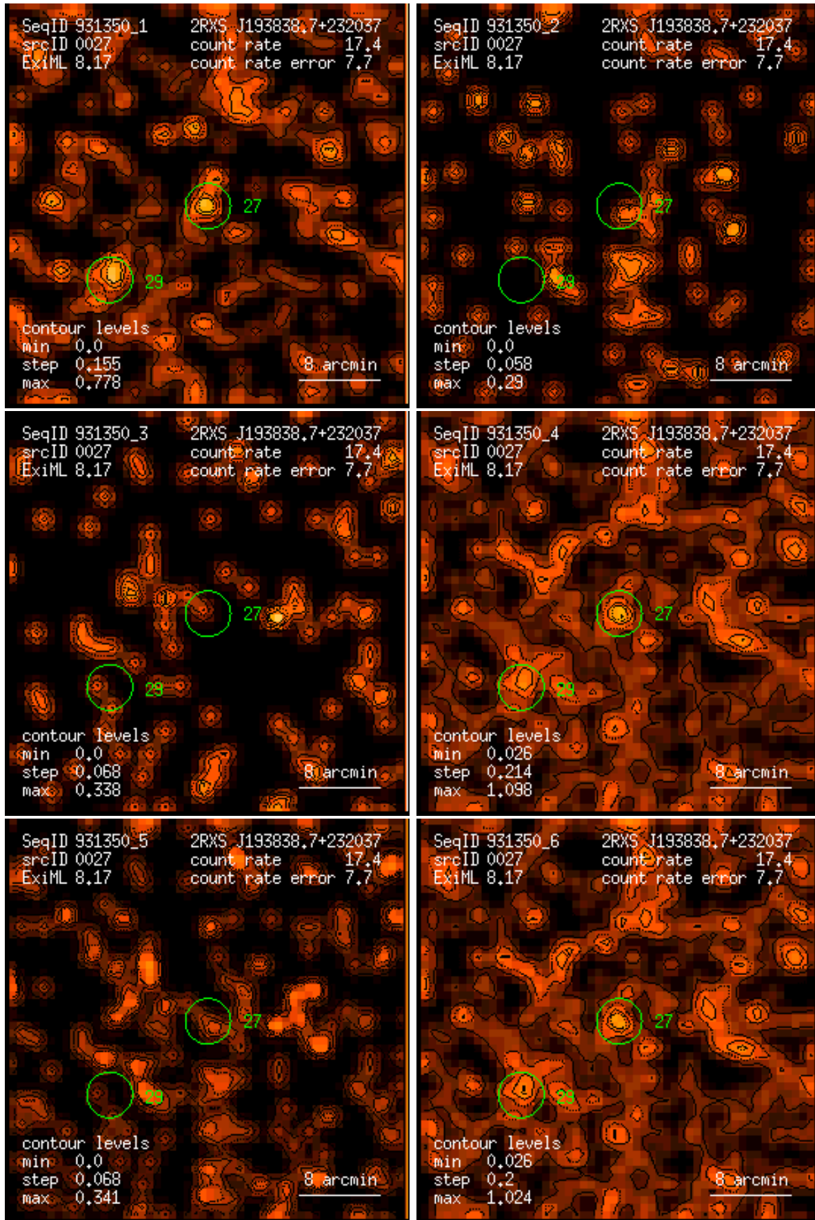
Figure 27: RASS 931350: detection 0027: band rate images, Gaussian filter: (1) PSPC channels 11 – 41, (2) 52 – 90, (3) 91 – 201, (4) 11 – 235, (5) 52 – 201, (6) 11 – 201. Broad band rates in counts/ks. Band rate contour levels in counts/ks/arcmin 2 .
