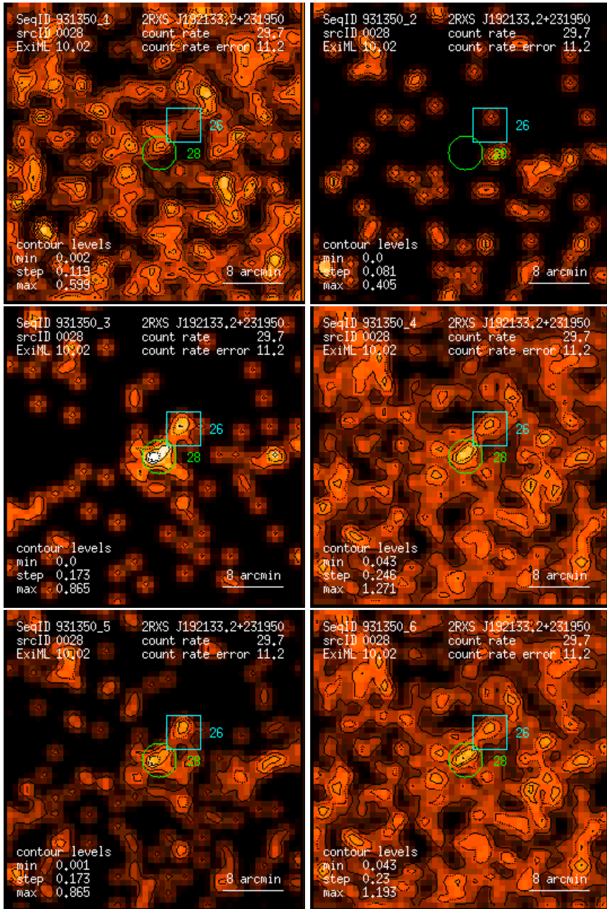
Figure 28: RASS 931350: detection 0028: band rate images, Gaussian filter: (1) PSPC channels 11 – 41, (2) 52 – 90, (3) 91 – 201, (4) 11 – 235, (5) 52 – 201, (6) 11 – 201. Broad band rates in counts/ks. Band rate contour levels in counts/ks/arcmin 2 .
