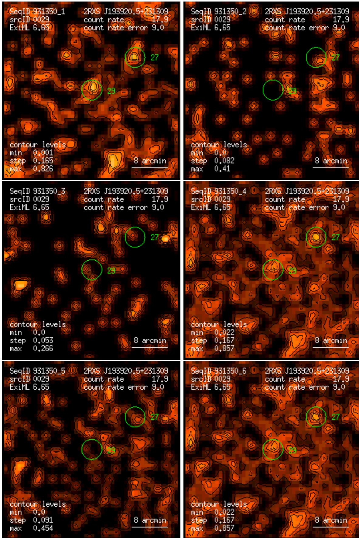
Figure 29: RASS 931350: detection 0029: band rate images, Gaussian filter: (1) PSPC channels 11 – 41, (2) 52 – 90, (3) 91 – 201, (4) 11 – 235, (5) 52 – 201, (6) 11 – 201. Broad band rates in counts/ks. Band rate contour levels in counts/ks/arcmin 2 .
