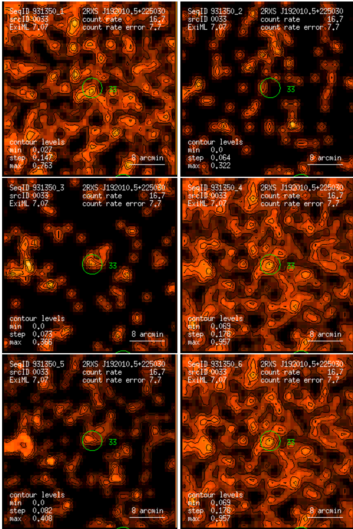
Figure 33: RASS 931350: detection 0033: band rate images, Gaussian filter: (1) PSPC channels 11 – 41, (2) 52 – 90, (3) 91 – 201, (4) 11 – 235, (5) 52 – 201, (6) 11 – 201. Broad band rates in counts/ks. Band rate contour levels in counts/ks/arcmin 2 .
