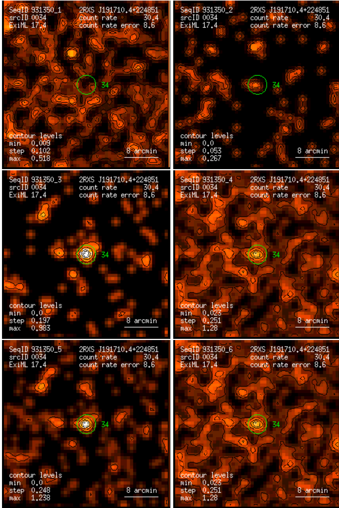
Figure 34: RASS 931350: detection 0034: band rate images, Gaussian filter: (1) PSPC channels 11 – 41, (2) 52 – 90, (3) 91 – 201, (4) 11 – 235, (5) 52 – 201, (6) 11 – 201. Broad band rates in counts/ks. Band rate contour levels in counts/ks/arcmin 2 .
