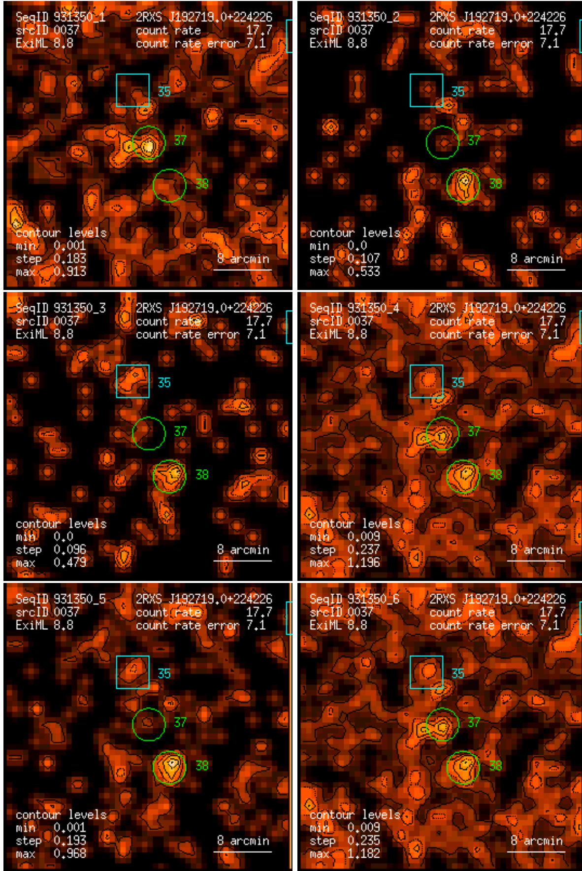
Figure 37: RASS 931350: detection 0037: band rate images, Gaussian filter: (1) PSPC channels 11 – 41, (2) 52 – 90, (3) 91 – 201, (4) 11 – 235, (5) 52 – 201, (6) 11 – 201. Broad band rates in counts/ks. Band rate contour levels in counts/ks/arcmin 2 .
