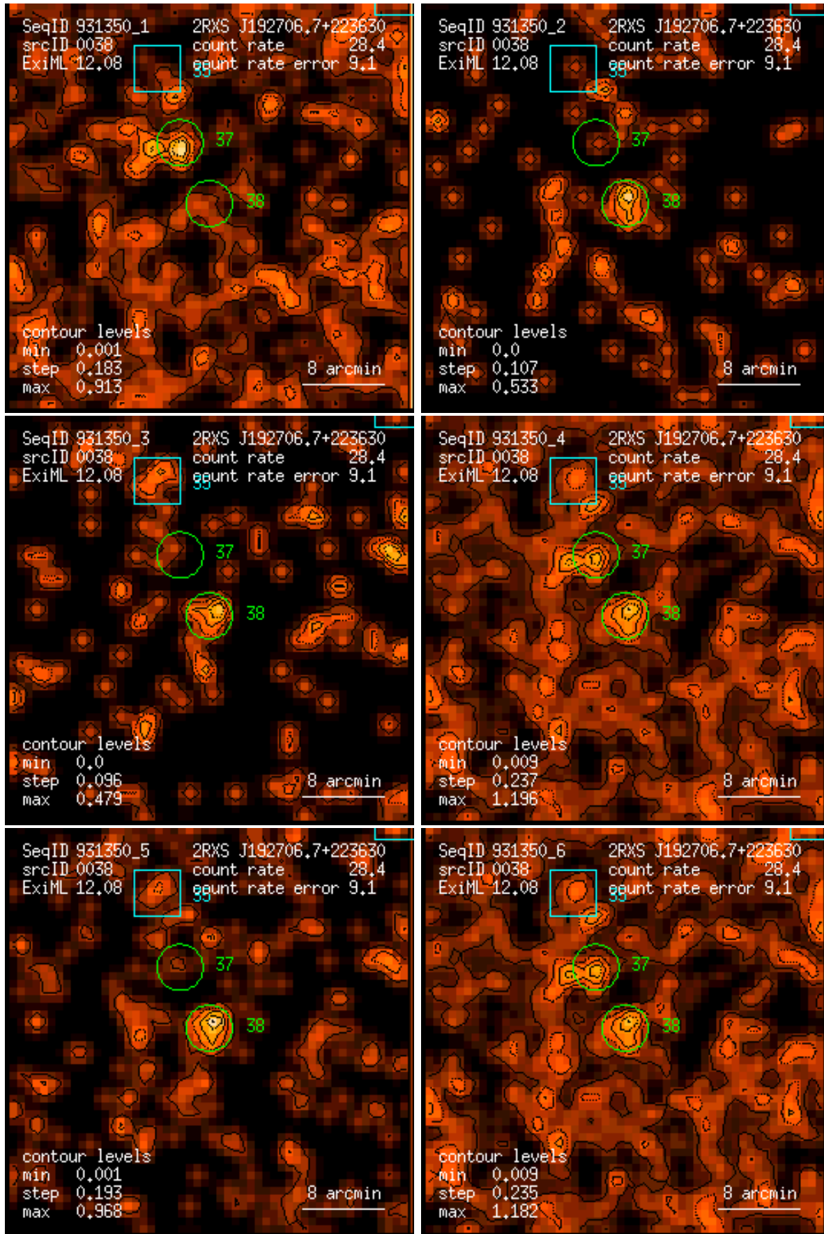
Figure 38: RASS 931350: detection 0038: band rate images, Gaussian filter: (1) PSPC channels 11 – 41, (2) 52 – 90, (3) 91 – 201, (4) 11 – 235, (5) 52 – 201, (6) 11 – 201. Broad band rates in counts/ks. Band rate contour levels in counts/ks/arcmin 2 .
