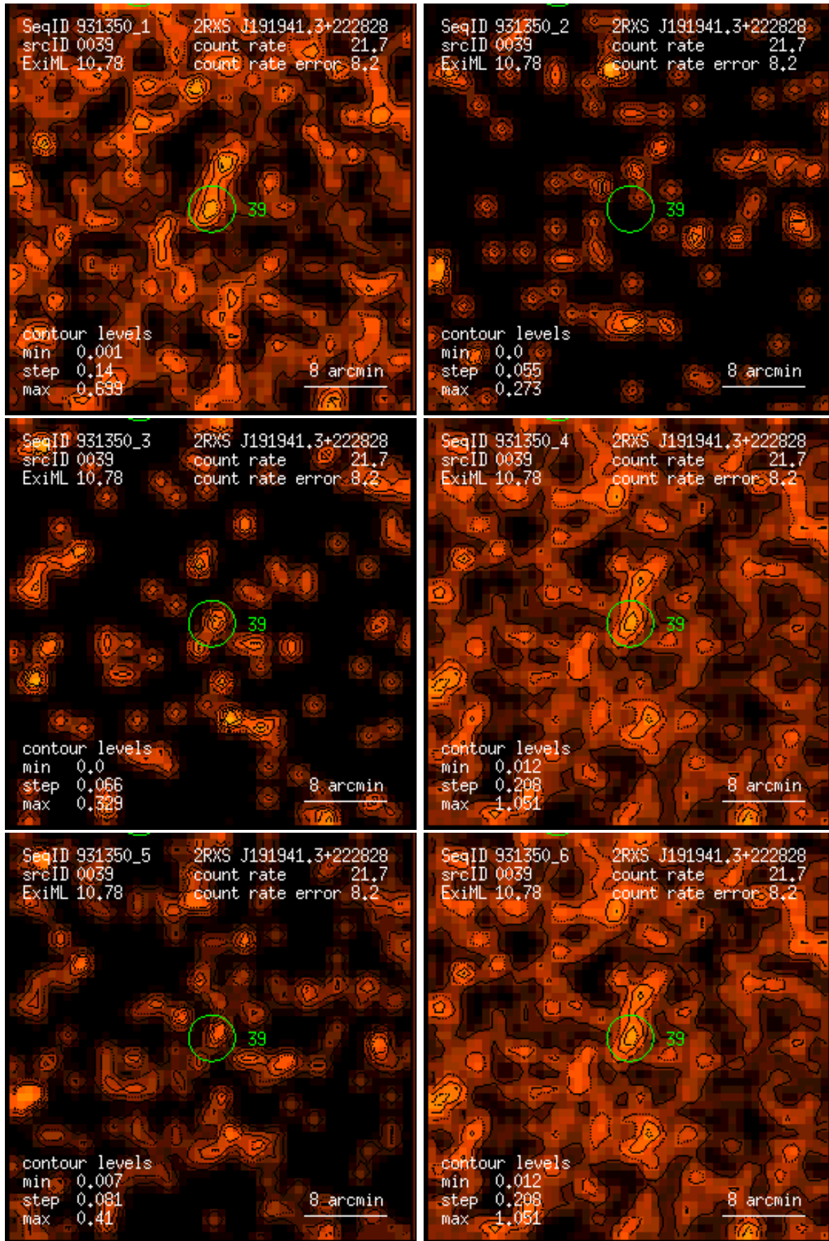
Figure 39: RASS 931350: detection 0039: band rate images, Gaussian filter: (1) PSPC channels 11 – 41, (2) 52 – 90, (3) 91 – 201, (4) 11 – 235, (5) 52 – 201, (6) 11 – 201. Broad band rates in counts/ks. Band rate contour levels in counts/ks/arcmin 2 .
