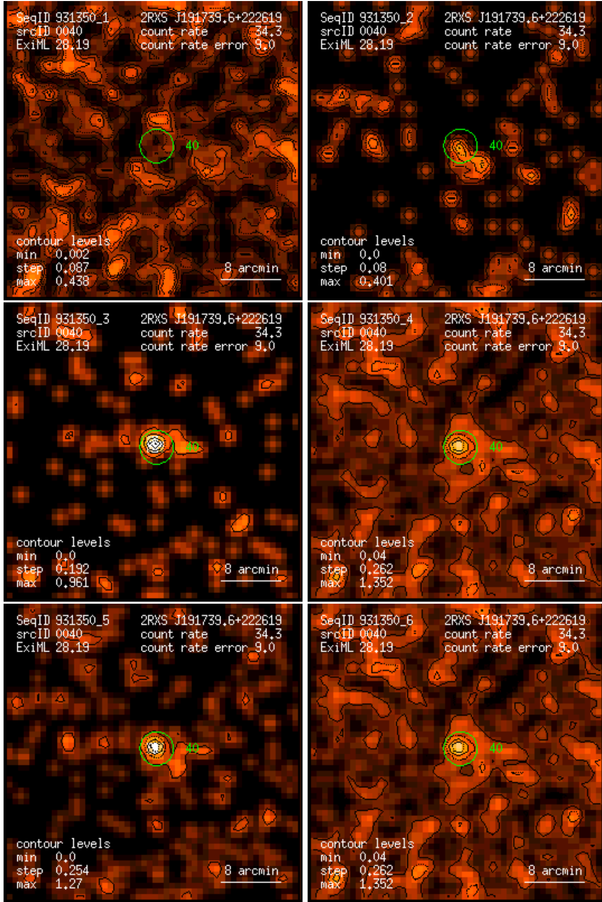
Figure 40: RASS 931350: detection 0040: band rate images, Gaussian filter: (1) PSPC channels 11 – 41, (2) 52 – 90, (3) 91 – 201, (4) 11 – 235, (5) 52 – 201, (6) 11 – 201. Broad band rates in counts/ks. Band rate contour levels in counts/ks/arcmin 2 .
