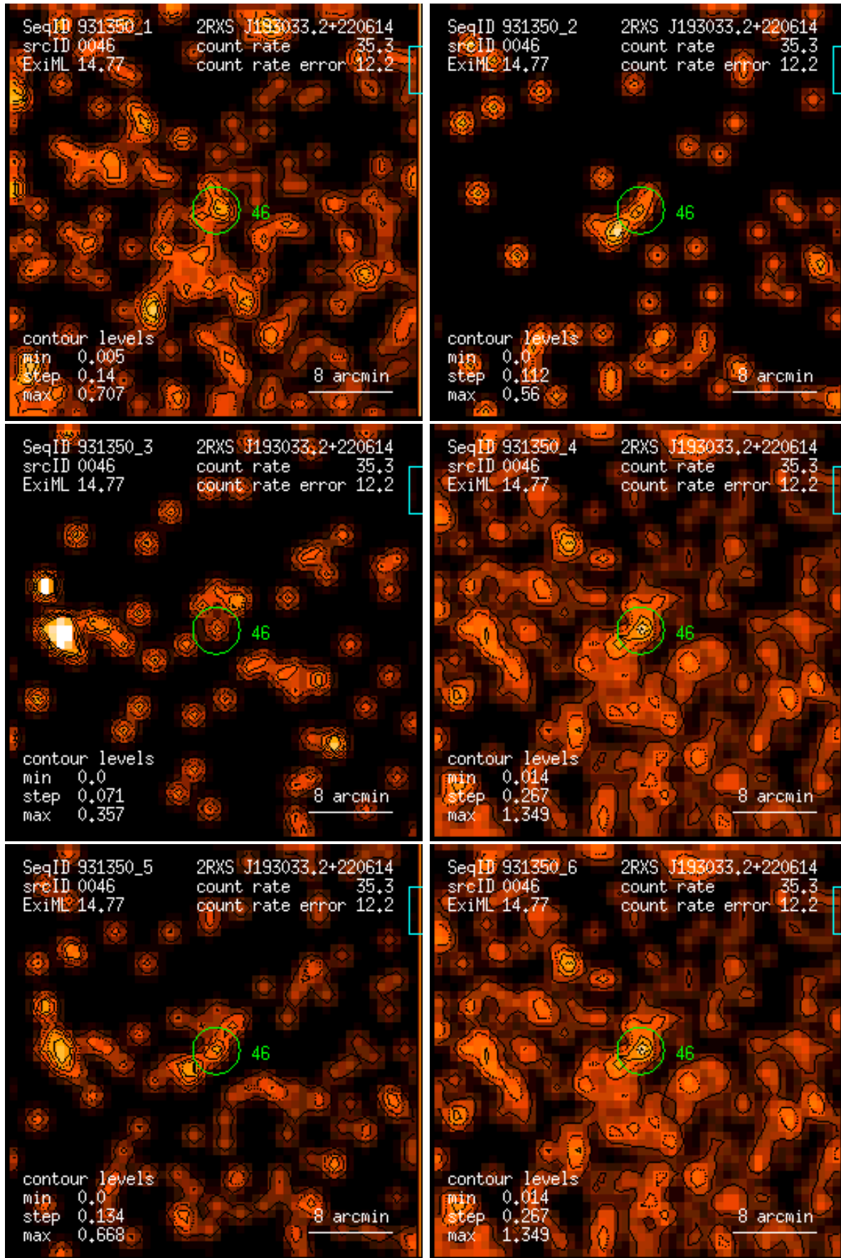
Figure 46: RASS 931350: detection 0046: band rate images, Gaussian filter: (1) PSPC channels 11 – 41, (2) 52 – 90, (3) 91 – 201, (4) 11 – 235, (5) 52 – 201, (6) 11 – 201. Broad band rates in counts/ks. Band rate contour levels in counts/ks/arcmin 2 .
