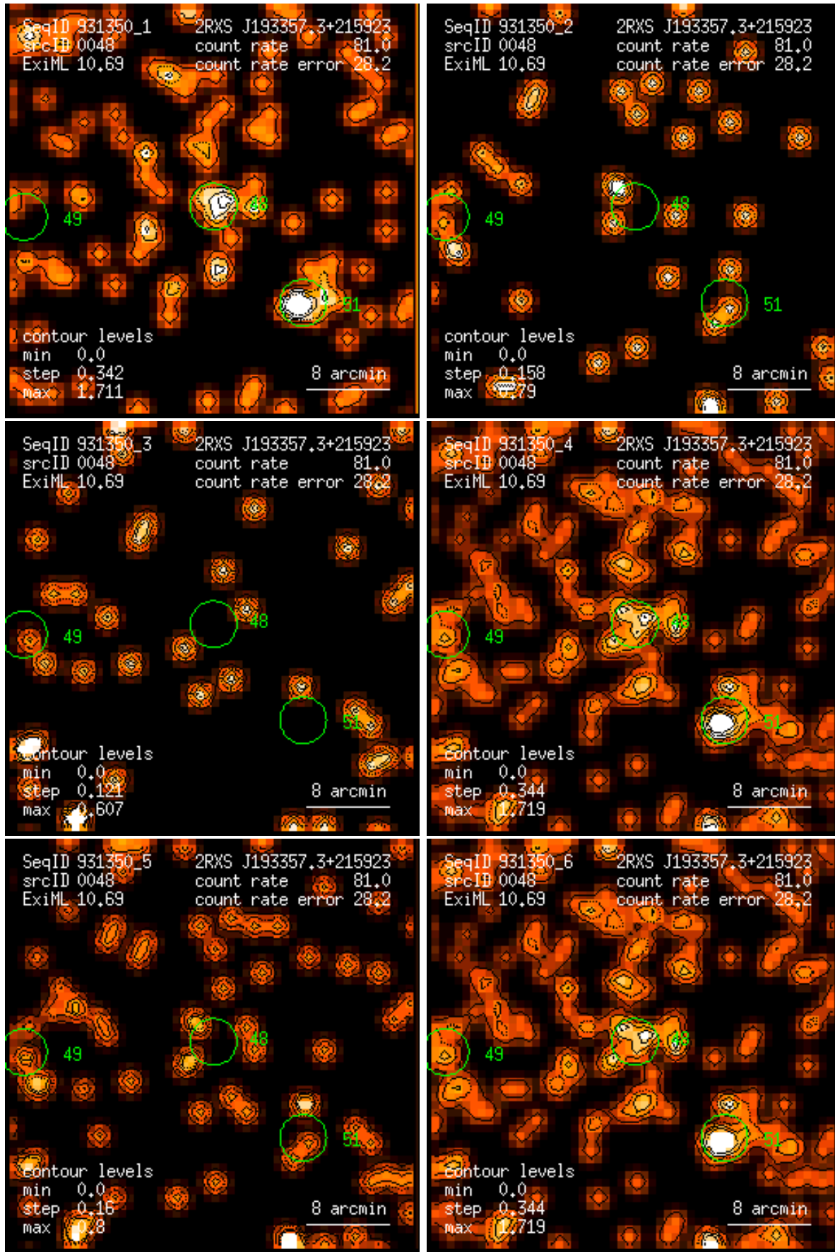
Figure 48: RASS 931350: detection 0048: band rate images, Gaussian filter: (1) PSPC channels 11 – 41, (2) 52 – 90, (3) 91 – 201, (4) 11 – 235, (5) 52 – 201, (6) 11 – 201. Broad band rates in counts/ks. Band rate contour levels in counts/ks/arcmin 2 .
