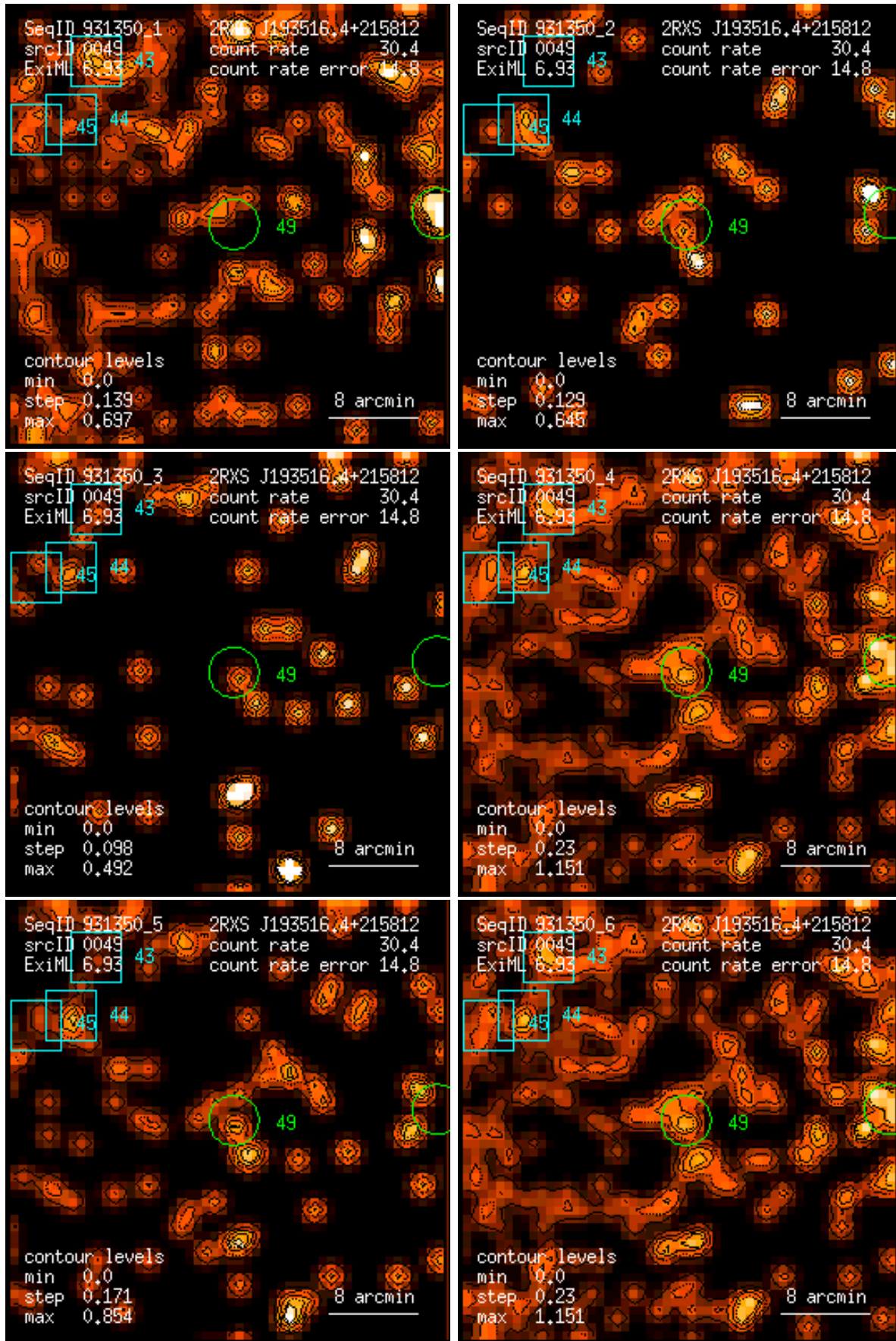
Figure 49: RASS 931350: detection 0049: band rate images, Gaussian filter: (1) PSPC channels 11 – 41, (2) 52 – 90, (3) 91 – 201, (4) 11 – 235, (5) 52 – 201, (6) 11 – 201. Broad band rates in counts/ks. Band rate contour levels in counts/ks/arcmin 2 .
