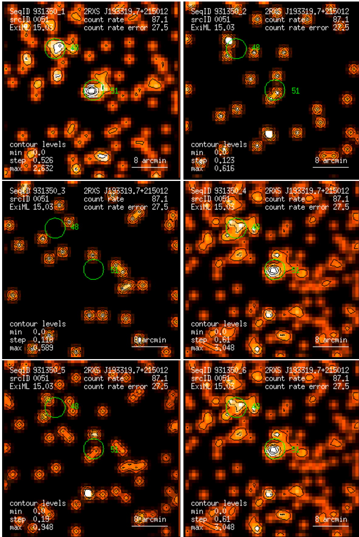
Figure 51: RASS 931350: detection 0051: band rate images, Gaussian filter: (1) PSPC channels 11 – 41, (2) 52 – 90, (3) 91 – 201, (4) 11 – 235, (5) 52 – 201, (6) 11 – 201. Broad band rates in counts/ks. Band rate contour levels in counts/ks/arcmin 2 .
