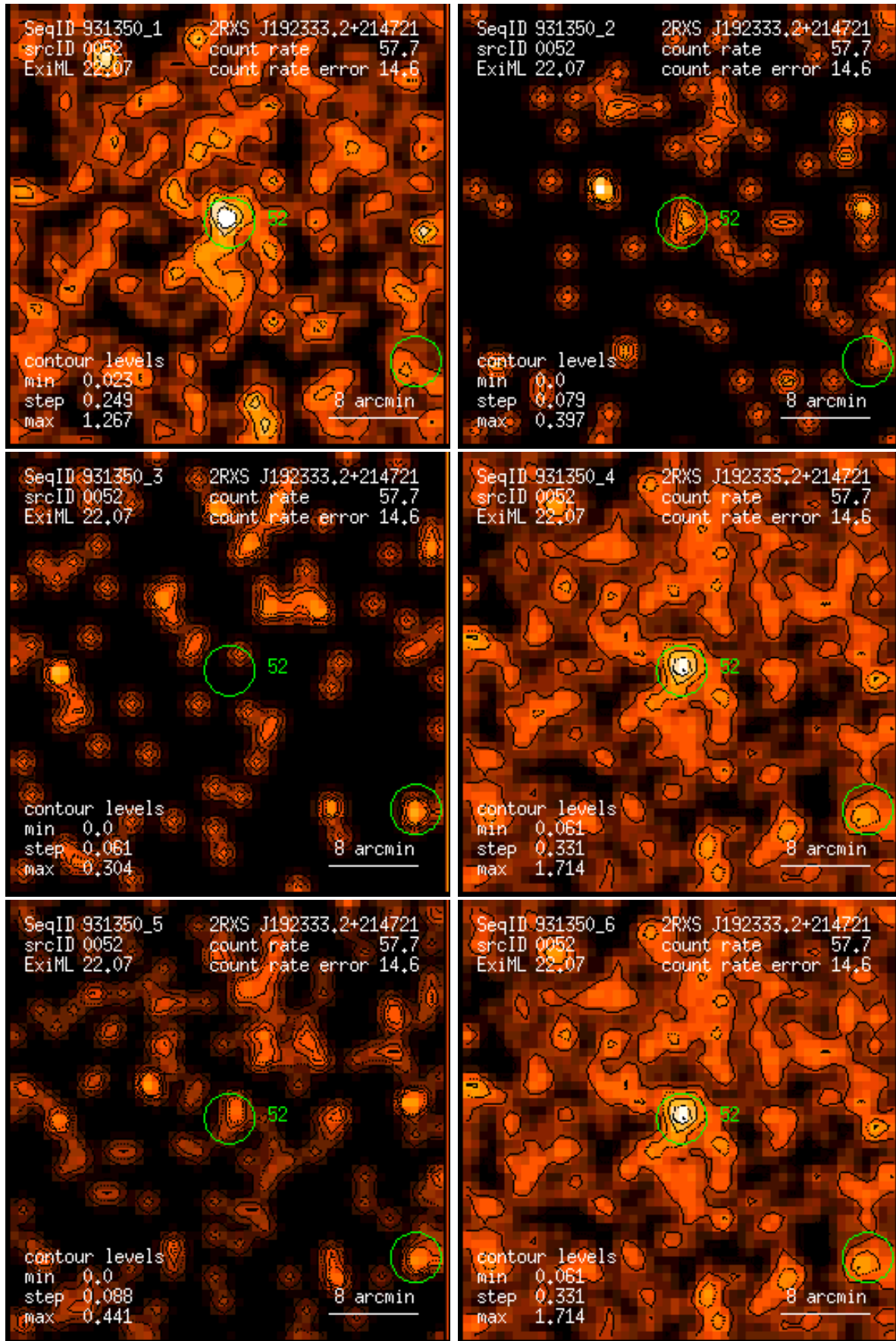
Figure 52: RASS 931350: detection 0052: band rate images, Gaussian filter: (1) PSPC channels 11 – 41, (2) 52 – 90, (3) 91 – 201, (4) 11 – 235, (5) 52 – 201, (6) 11 – 201. Broad band rates in counts/ks. Band rate contour levels in counts/ks/arcmin 2 .
