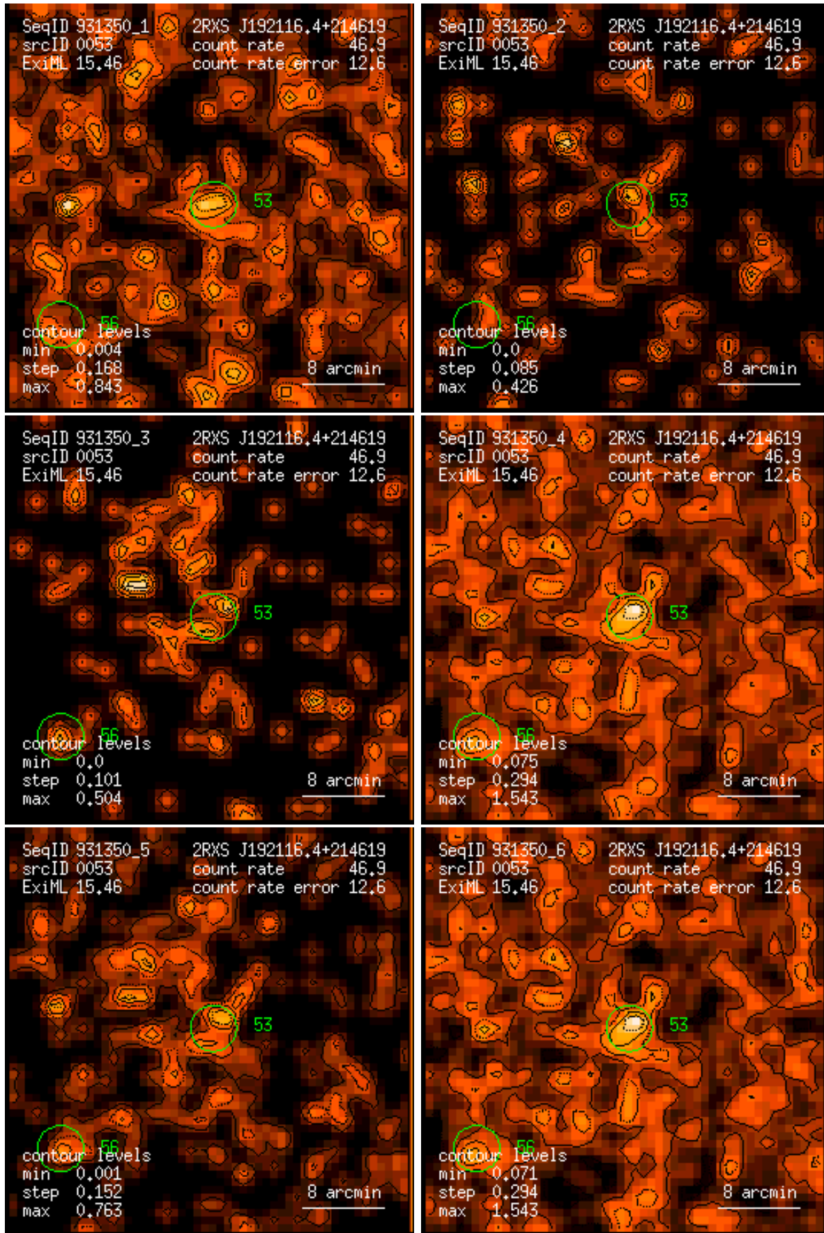
Figure 53: RASS 931350: detection 0053: band rate images, Gaussian filter: (1) PSPC channels 11 – 41, (2) 52 – 90, (3) 91 – 201, (4) 11 – 235, (5) 52 – 201, (6) 11 – 201. Broad band rates in counts/ks. Band rate contour levels in counts/ks/arcmin 2 .
