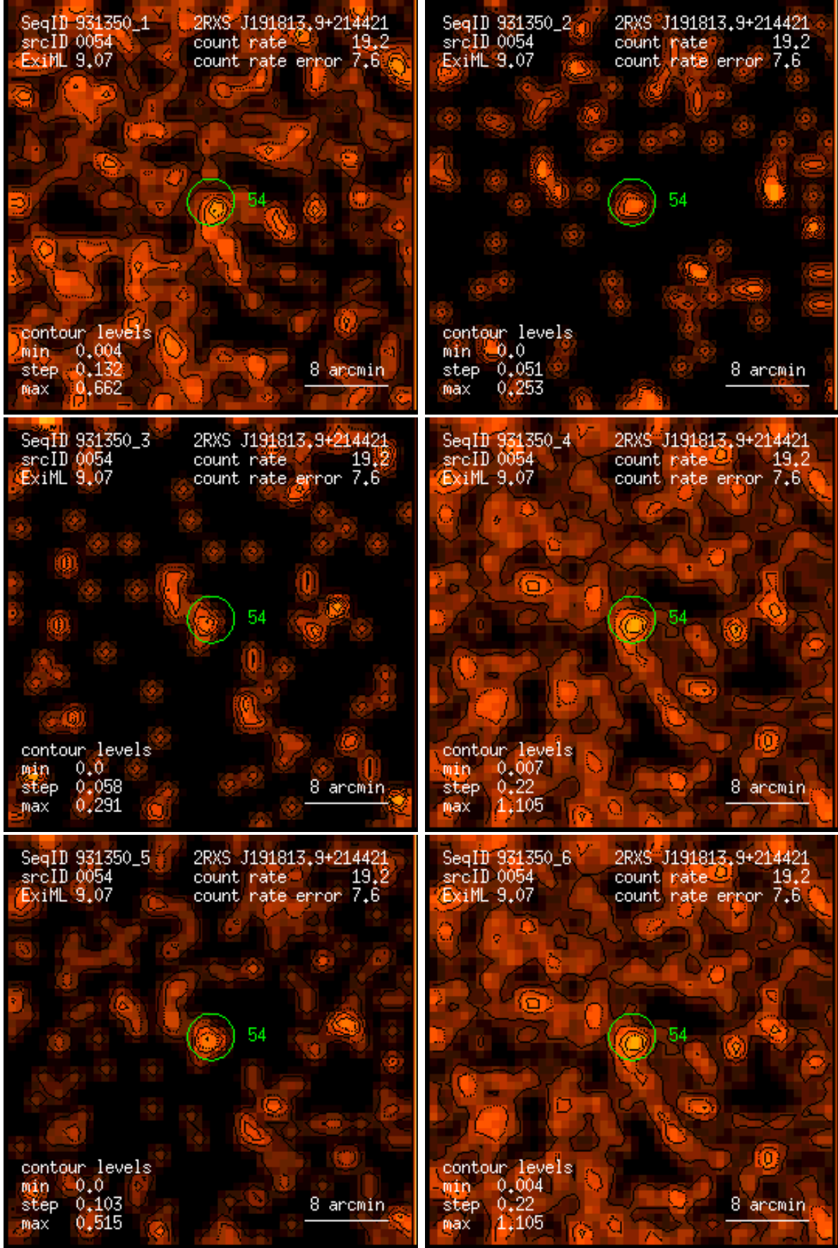
Figure 54: RASS 931350: detection 0054: band rate images, Gaussian filter: (1) PSPC channels 11 – 41, (2) 52 – 90, (3) 91 – 201, (4) 11 – 235, (5) 52 – 201, (6) 11 – 201. Broad band rates in counts/ks. Band rate contour levels in counts/ks/arcmin 2 .
