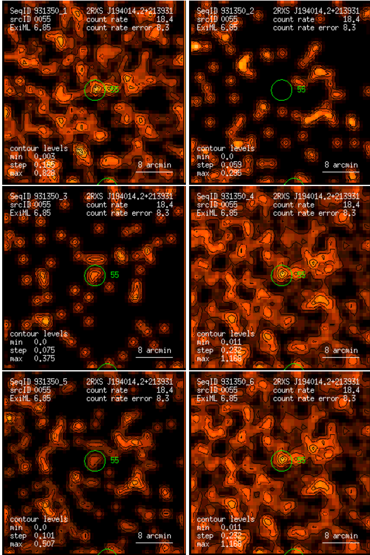
Figure 55: RASS 931350: detection 0055: band rate images, Gaussian filter: (1) PSPC channels 11 – 41, (2) 52 – 90, (3) 91 – 201, (4) 11 – 235, (5) 52 – 201, (6) 11 – 201. Broad band rates in counts/ks. Band rate contour levels in counts/ks/arcmin 2 .
