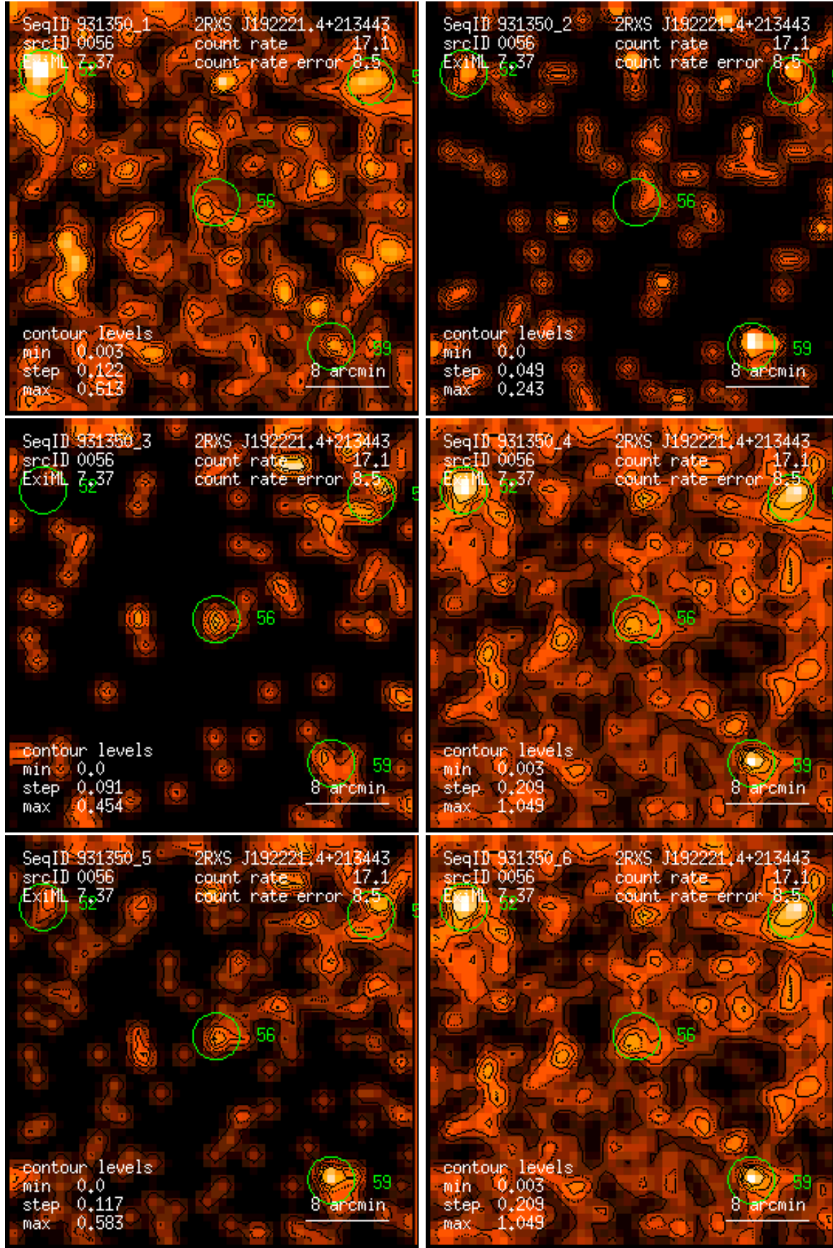
Figure 56: RASS 931350: detection 0056: band rate images, Gaussian filter: (1) PSPC channels 11 – 41, (2) 52 – 90, (3) 91 – 201, (4) 11 – 235, (5) 52 – 201, (6) 11 – 201. Broad band rates in counts/ks. Band rate contour levels in counts/ks/arcmin 2 .
