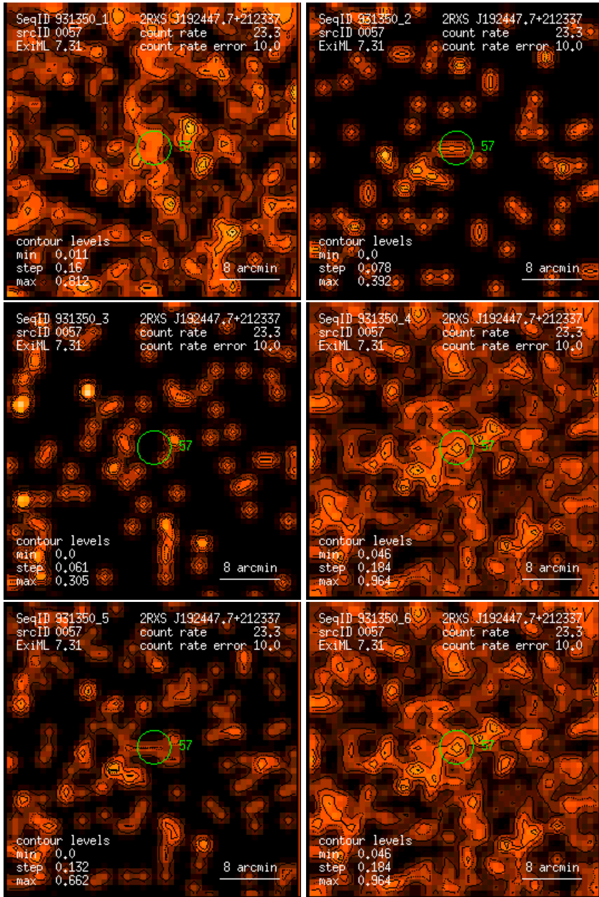
Figure 57: RASS 931350: detection 0057: band rate images, Gaussian filter: (1) PSPC channels 11 – 41, (2) 52 – 90, (3) 91 – 201, (4) 11 – 235, (5) 52 – 201, (6) 11 – 201. Broad band rates in counts/ks. Band rate contour levels in counts/ks/arcmin 2 .
