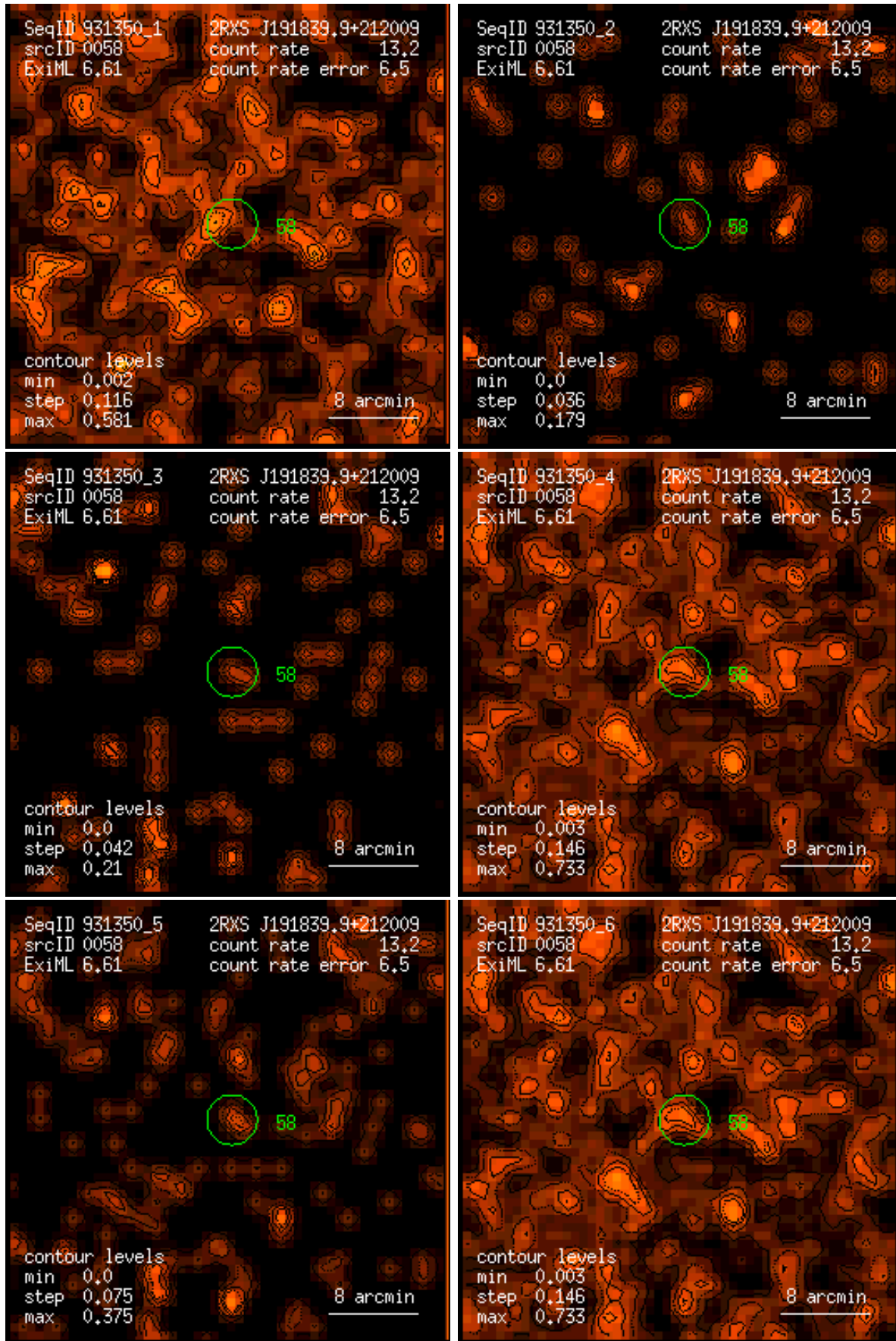
Figure 58: RASS 931350: detection 0058: band rate images, Gaussian filter: (1) PSPC channels 11 – 41, (2) 52 – 90, (3) 91 – 201, (4) 11 – 235, (5) 52 – 201, (6) 11 – 201. Broad band rates in counts/ks. Band rate contour levels in counts/ks/arcmin 2 .
