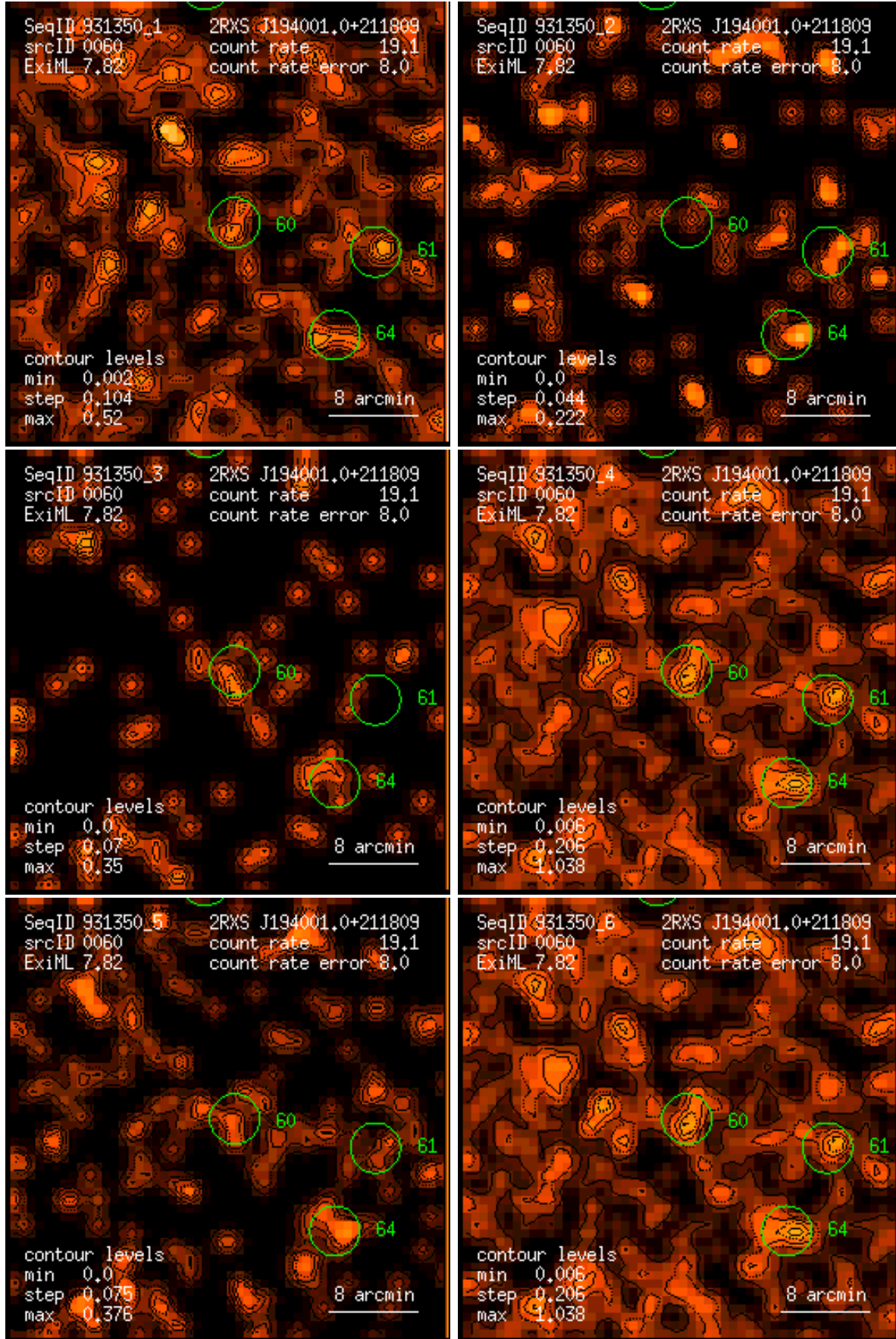
Figure 60: RASS 931350: detection 0060: band rate images, Gaussian filter: (1) PSPC channels 11 – 41, (2) 52 – 90, (3) 91 – 201, (4) 11 – 235, (5) 52 – 201, (6) 11 – 201. Broad band rates in counts/ks. Band rate contour levels in counts/ks/arcmin 2 .
