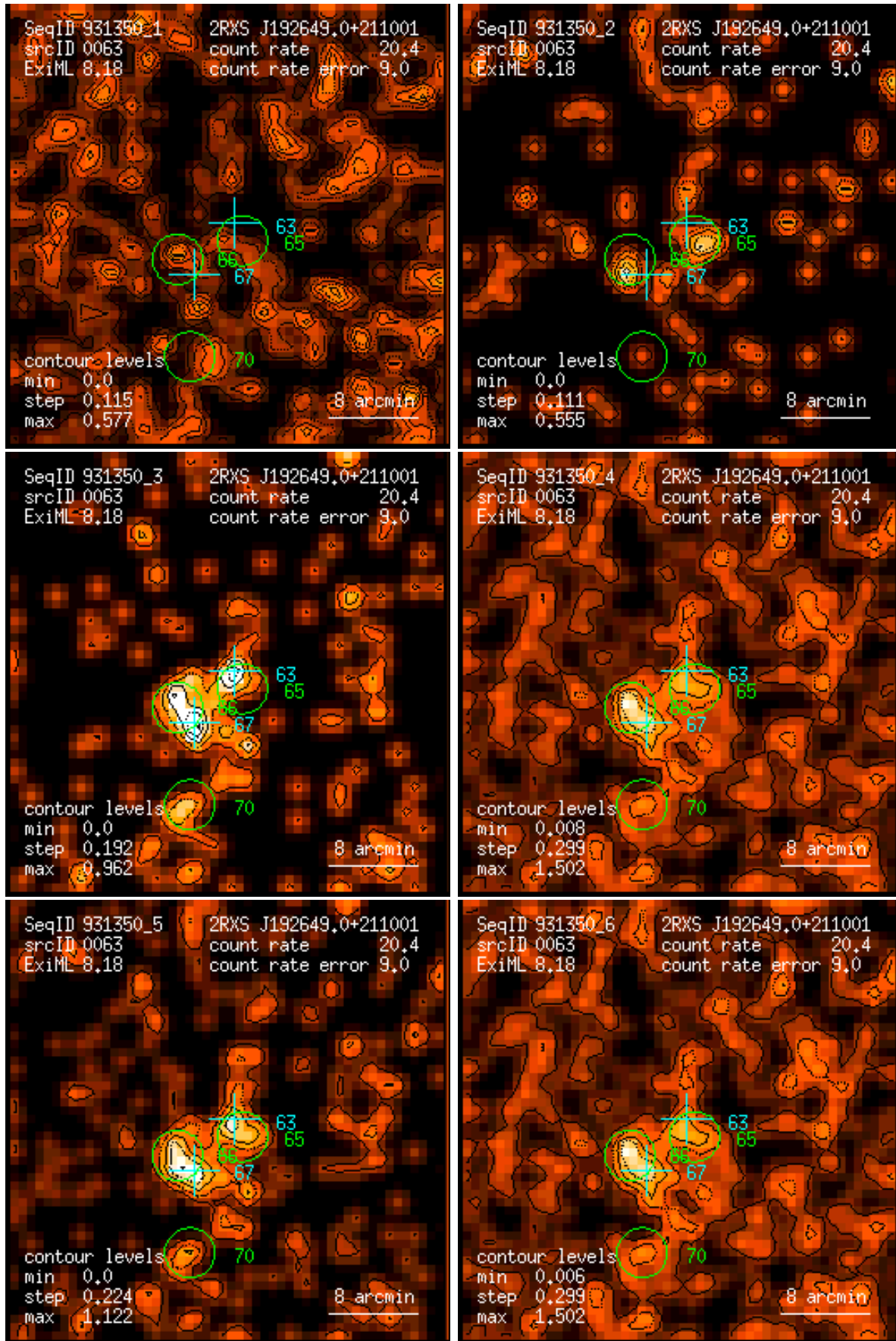
Figure 63: RASS 931350: detection 0063: band rate images, Gaussian filter: (1) PSPC channels 11 – 41, (2) 52 – 90, (3) 91 – 201, (4) 11 – 235, (5) 52 – 201, (6) 11 – 201. Broad band rates in counts/ks. Band rate contour levels in counts/ks/arcmin 2 .
