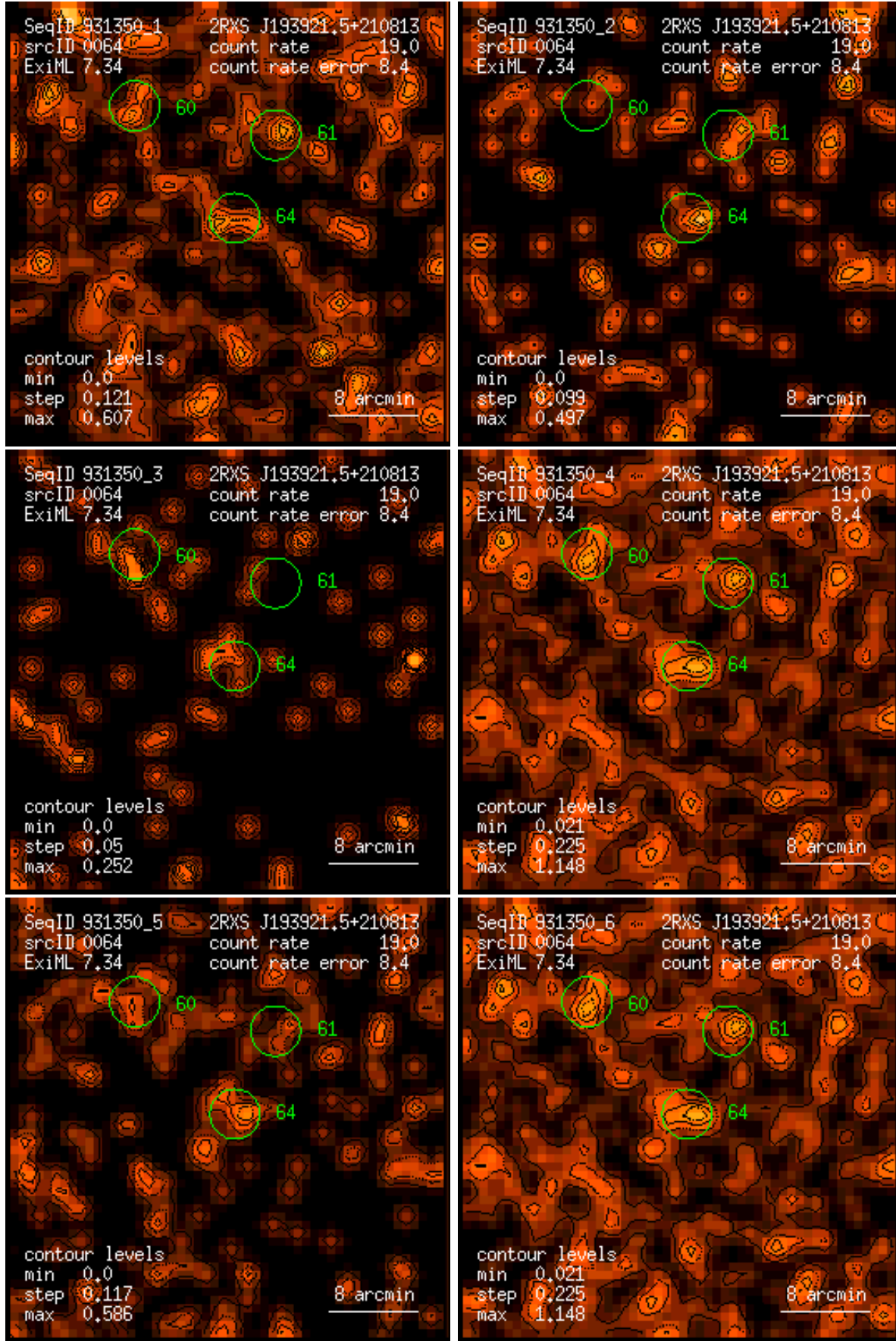
Figure 64: RASS 931350: detection 0064: band rate images, Gaussian filter: (1) PSPC channels 11 – 41, (2) 52 – 90, (3) 91 – 201, (4) 11 – 235, (5) 52 – 201, (6) 11 – 201. Broad band rates in counts/ks. Band rate contour levels in counts/ks/arcmin 2 .
