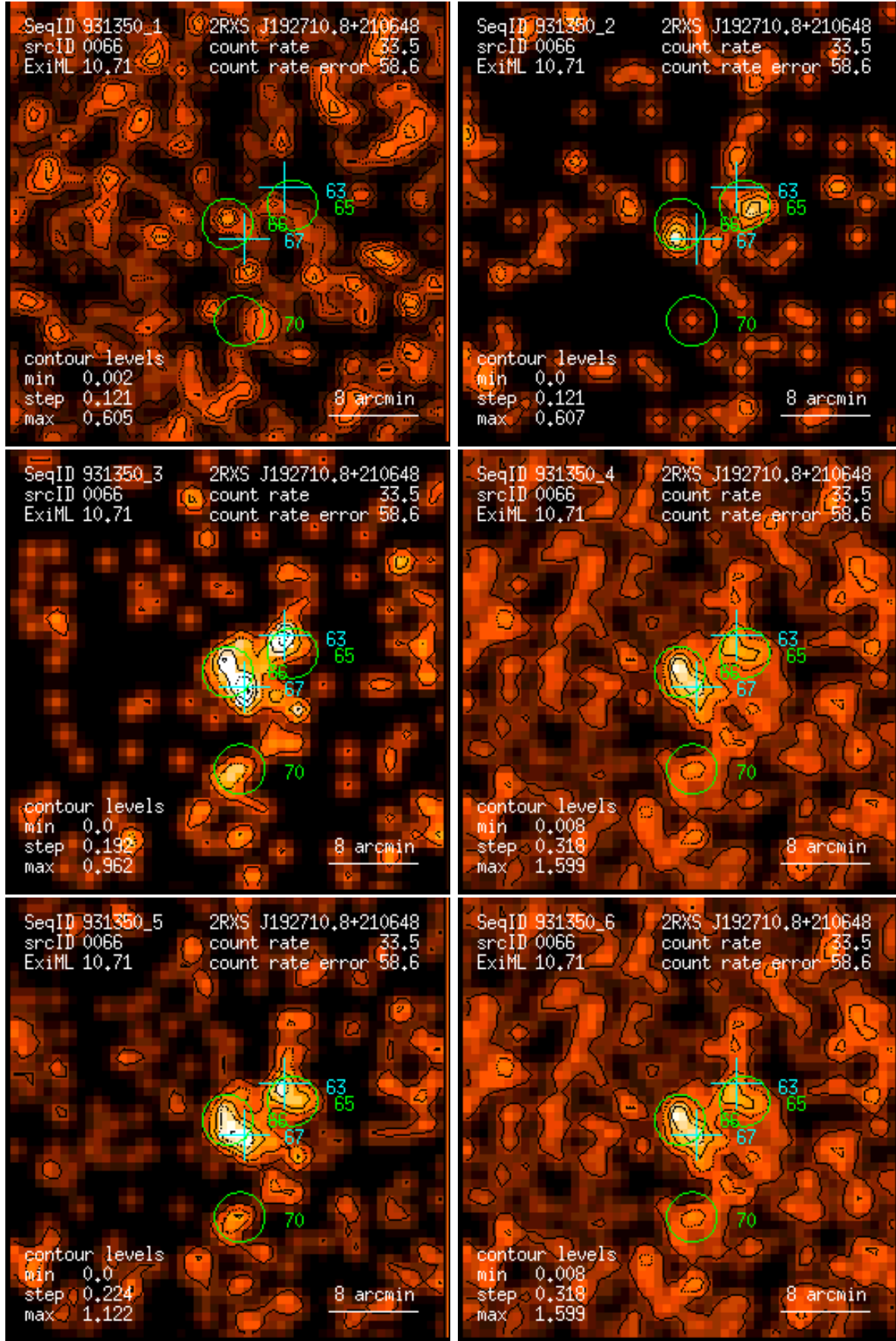
Figure 66: RASS 931350: detection 0066: band rate images, Gaussian filter: (1) PSPC channels 11 – 41, (2) 52 – 90, (3) 91 – 201, (4) 11 – 235, (5) 52 – 201, (6) 11 – 201. Broad band rates in counts/ks. Band rate contour levels in counts/ks/arcmin 2 .
