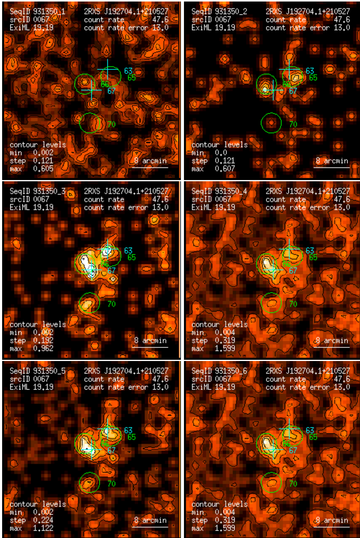
Figure 67: RASS 931350: detection 0067: band rate images, Gaussian filter: (1) PSPC channels 11 – 41, (2) 52 – 90, (3) 91 – 201, (4) 11 – 235, (5) 52 – 201, (6) 11 – 201. Broad band rates in counts/ks. Band rate contour levels in counts/ks/arcmin 2 .
