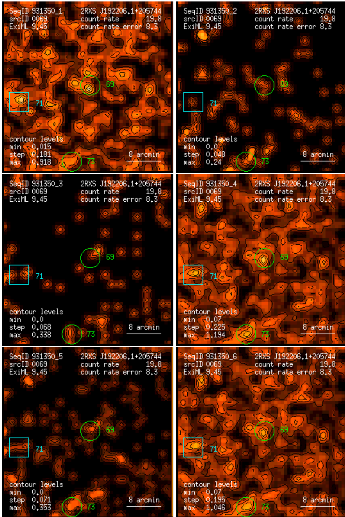
Figure 69: RASS 931350: detection 0069: band rate images, Gaussian filter: (1) PSPC channels 11 – 41, (2) 52 – 90, (3) 91 – 201, (4) 11 – 235, (5) 52 – 201, (6) 11 – 201. Broad band rates in counts/ks. Band rate contour levels in counts/ks/arcmin 2 .
