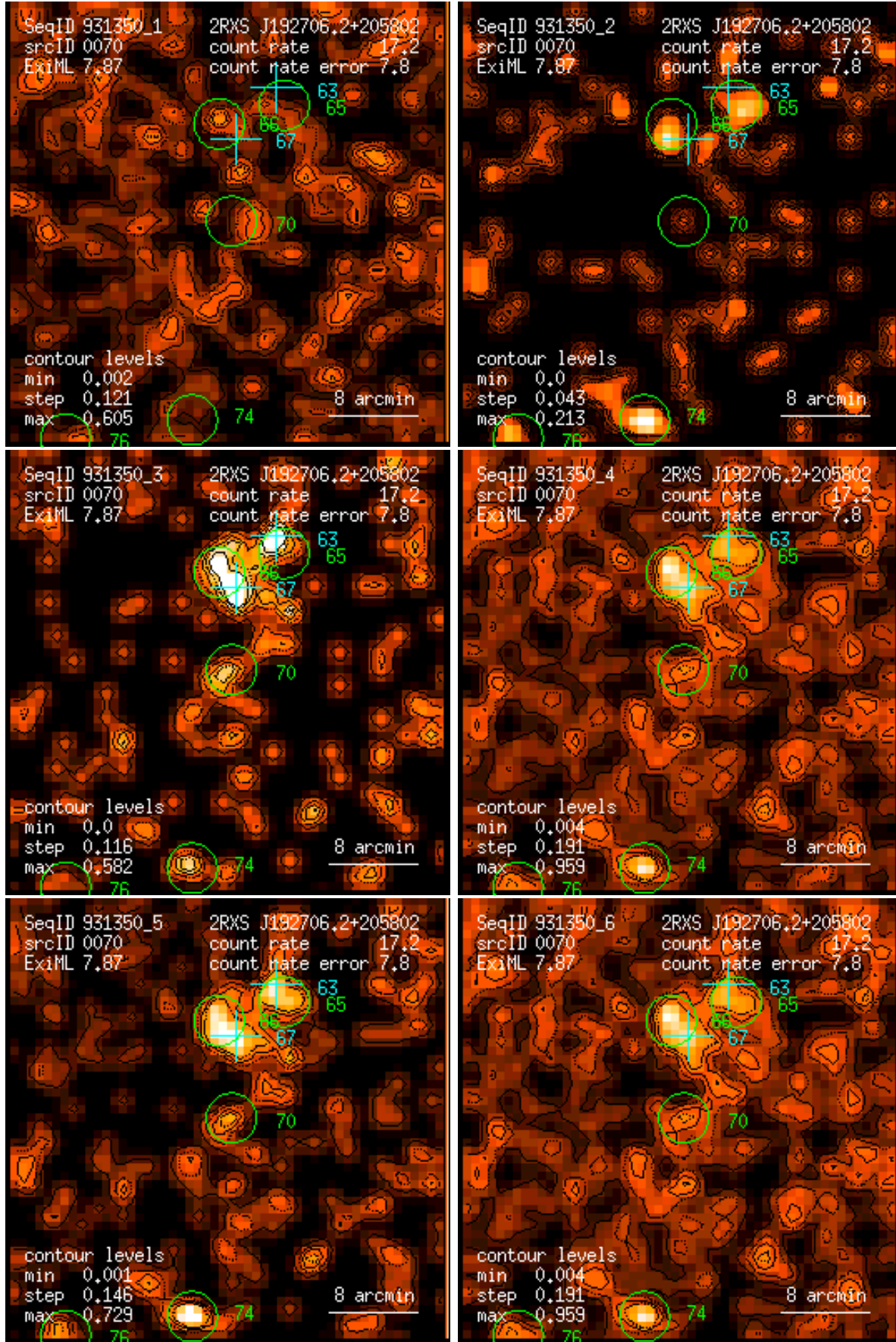
Figure 70: RASS 931350: detection 0070: band rate images, Gaussian filter: (1) PSPC channels 11 – 41, (2) 52 – 90, (3) 91 – 201, (4) 11 – 235, (5) 52 – 201, (6) 11 – 201. Broad band rates in counts/ks. Band rate contour levels in counts/ks/arcmin 2 .
