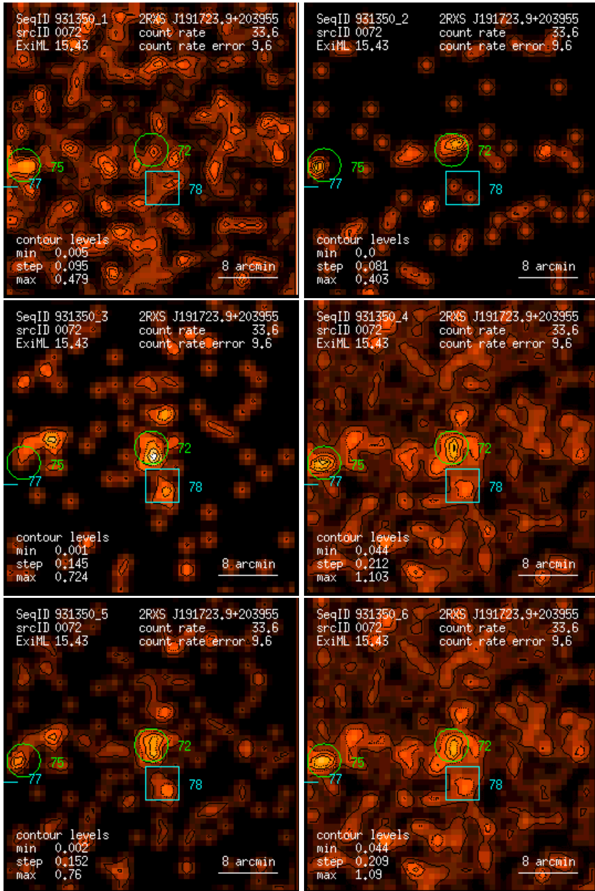
Figure 72: RASS 931350: detection 0072: band rate images, Gaussian filter: (1) PSPC channels 11 – 41, (2) 52 – 90, (3) 91 – 201, (4) 11 – 235, (5) 52 – 201, (6) 11 – 201. Broad band rates in counts/ks. Band rate contour levels in counts/ks/arcmin 2 .
