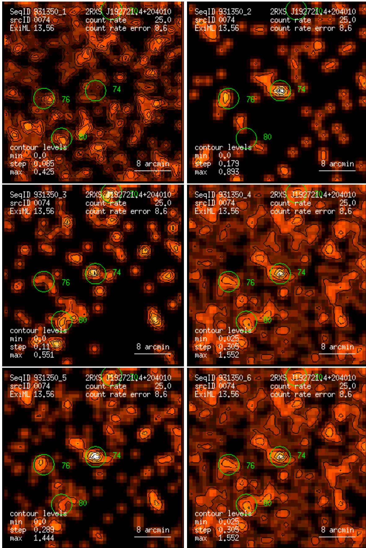
Figure 74: RASS 931350: detection 0074: band rate images, Gaussian filter: (1) PSPC channels 11 – 41, (2) 52 – 90, (3) 91 – 201, (4) 11 – 235, (5) 52 – 201, (6) 11 – 201. Broad band rates in counts/ks. Band rate contour levels in counts/ks/arcmin 2 .
