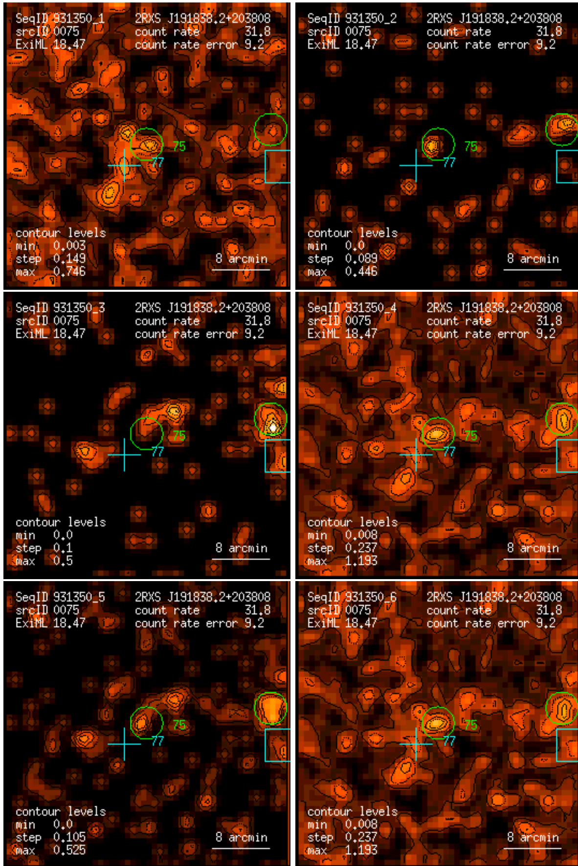
Figure 75: RASS 931350: detection 0075: band rate images, Gaussian filter: (1) PSPC channels 11 – 41, (2) 52 – 90, (3) 91 – 201, (4) 11 – 235, (5) 52 – 201, (6) 11 – 201. Broad band rates in counts/ks. Band rate contour levels in counts/ks/arcmin 2 .
