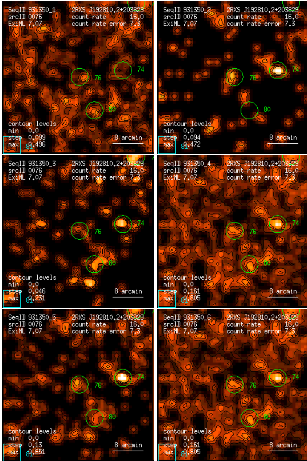
Figure 76: RASS 931350: detection 0076: band rate images, Gaussian filter: (1) PSPC channels 11 – 41, (2) 52 – 90, (3) 91 – 201, (4) 11 – 235, (5) 52 – 201, (6) 11 – 201. Broad band rates in counts/ks. Band rate contour levels in counts/ks/arcmin 2 .
