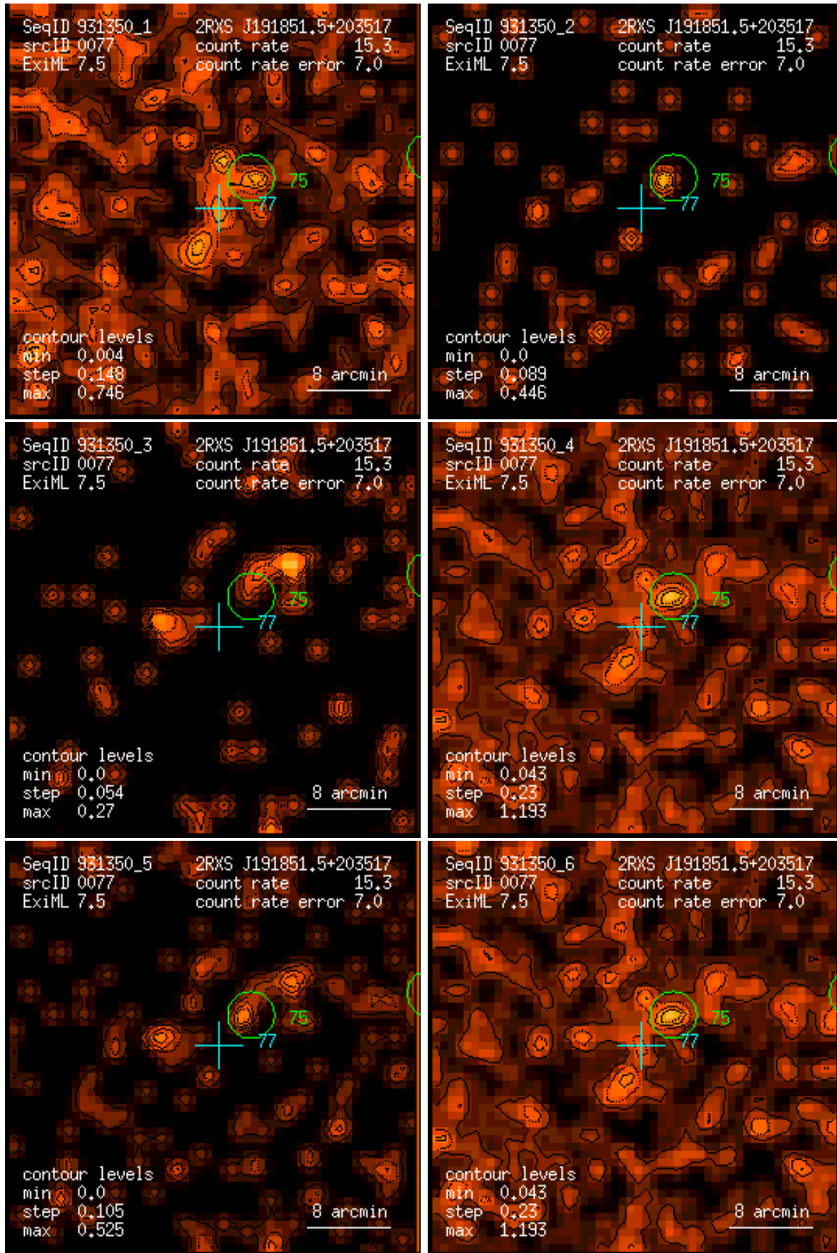
Figure 77: RASS 931350: detection 0077: band rate images, Gaussian filter: (1) PSPC channels 11 – 41, (2) 52 – 90, (3) 91 – 201, (4) 11 – 235, (5) 52 – 201, (6) 11 – 201. Broad band rates in counts/ks. Band rate contour levels in counts/ks/arcmin 2 .
