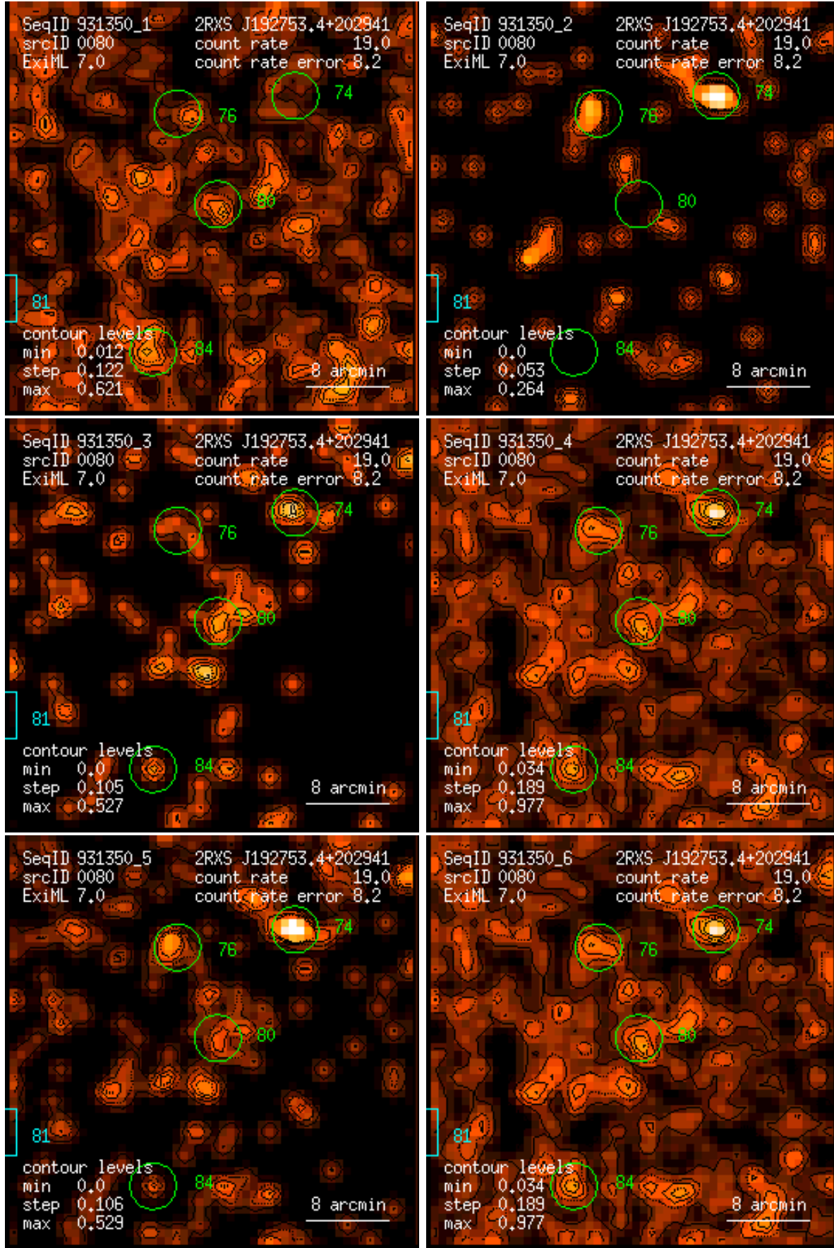
Figure 80: RASS 931350: detection 0080: band rate images, Gaussian filter: (1) PSPC channels 11 – 41, (2) 52 – 90, (3) 91 – 201, (4) 11 – 235, (5) 52 – 201, (6) 11 – 201. Broad band rates in counts/ks. Band rate contour levels in counts/ks/arcmin 2 .
