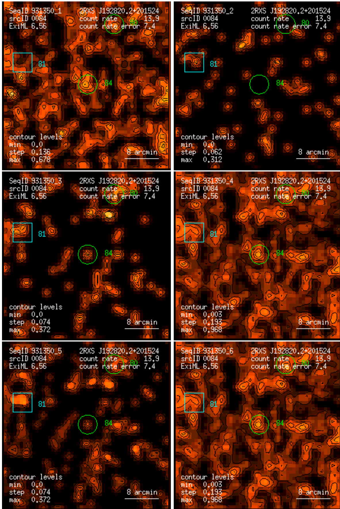
Figure 84: RASS 931350: detection 0084: band rate images, Gaussian filter: (1) PSPC channels 11 – 41, (2) 52 – 90, (3) 91 – 201, (4) 11 – 235, (5) 52 – 201, (6) 11 – 201. Broad band rates in counts/ks. Band rate contour levels in counts/ks/arcmin 2 .
