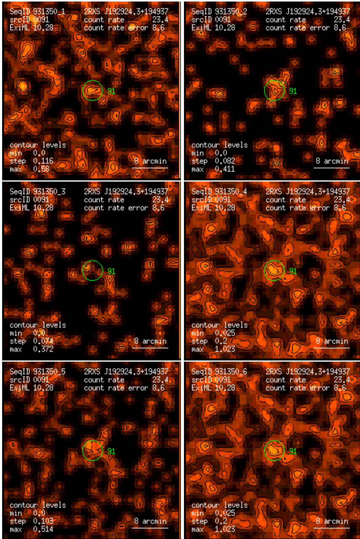
Figure 91: RASS 931350: detection 0091: band rate images, Gaussian filter: (1) PSPC channels 11 – 41, (2) 52 – 90, (3) 91 – 201, (4) 11 – 235, (5) 52 – 201, (6) 11 – 201. Broad band rates in counts/ks. Band rate contour levels in counts/ks/arcmin 2 .
