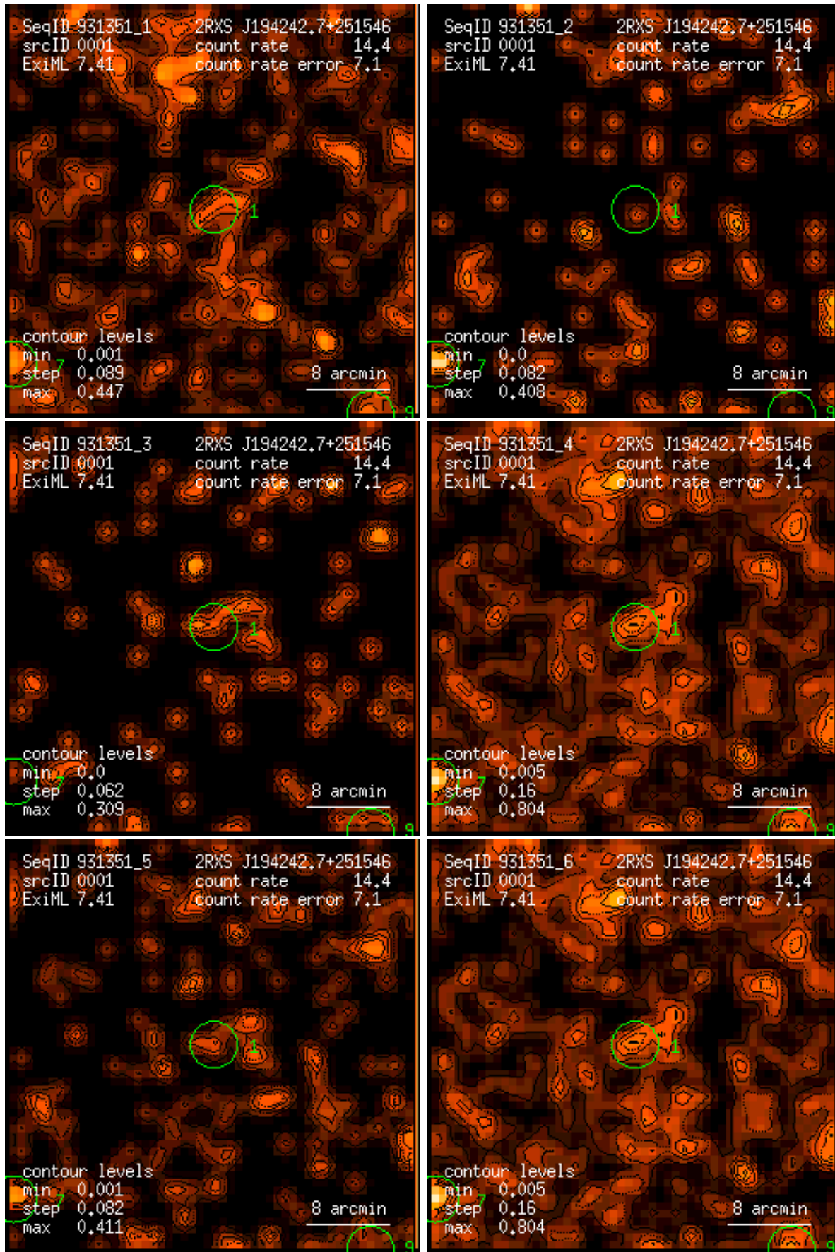
Figure 1: RASS 931351: detection 0001: band rate images, Gaussian filter: (1) PSPC channels 11 – 41, (2) 52 – 90, (3) 91 – 201, (4) 11 – 235, (5) 52 – 201, (6) 11 – 201. Broad band rates in counts/ks. Band rate contour levels in counts/ks/arcmin 2 .
