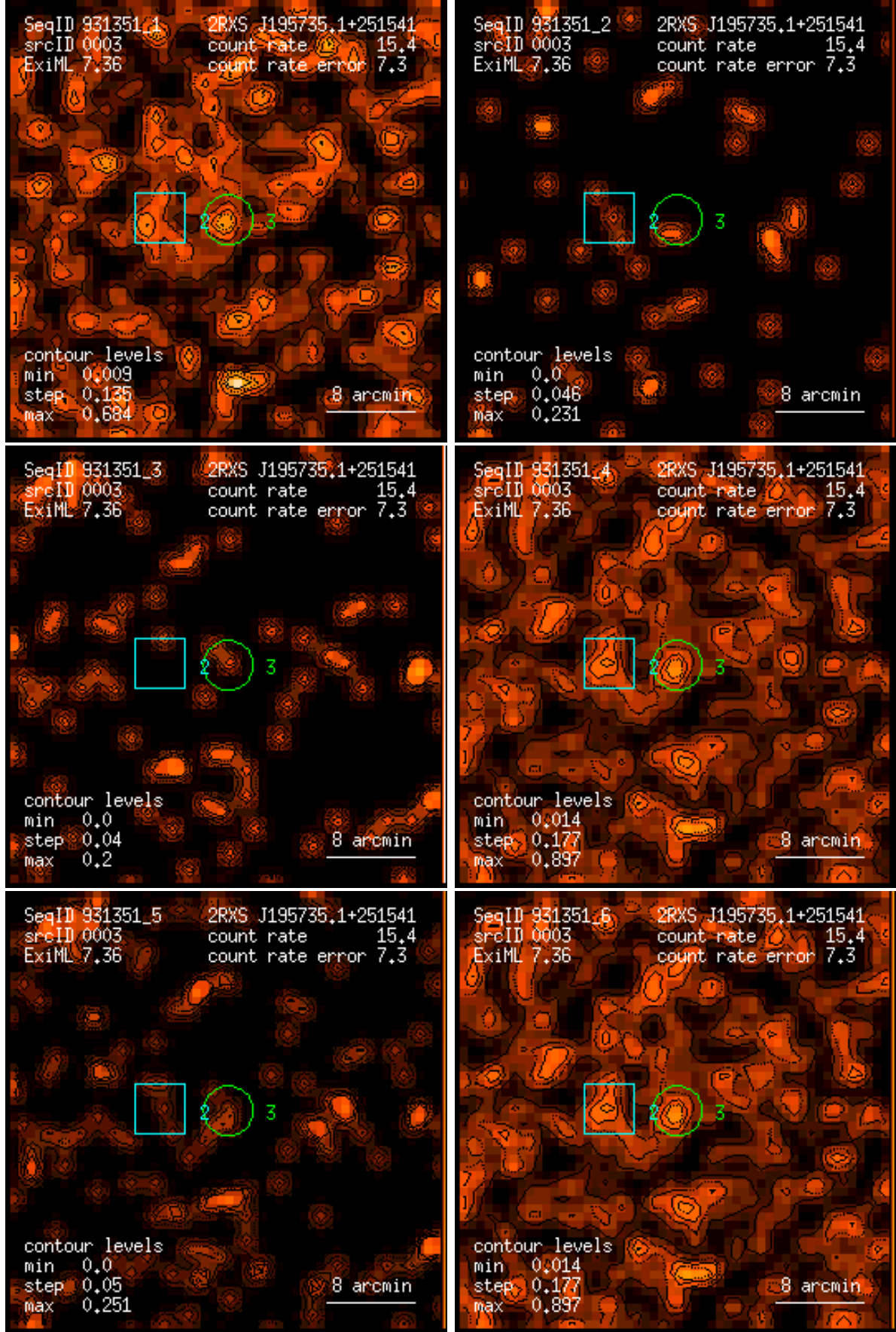
Figure 3: RASS 931351: detection 0003: band rate images, Gaussian filter: (1) PSPC channels 11 – 41, (2) 52 – 90, (3) 91 – 201, (4) 11 – 235, (5) 52 – 201, (6) 11 – 201. Broad band rates in counts/ks. Band rate contour levels in counts/ks/arcmin 2 .
