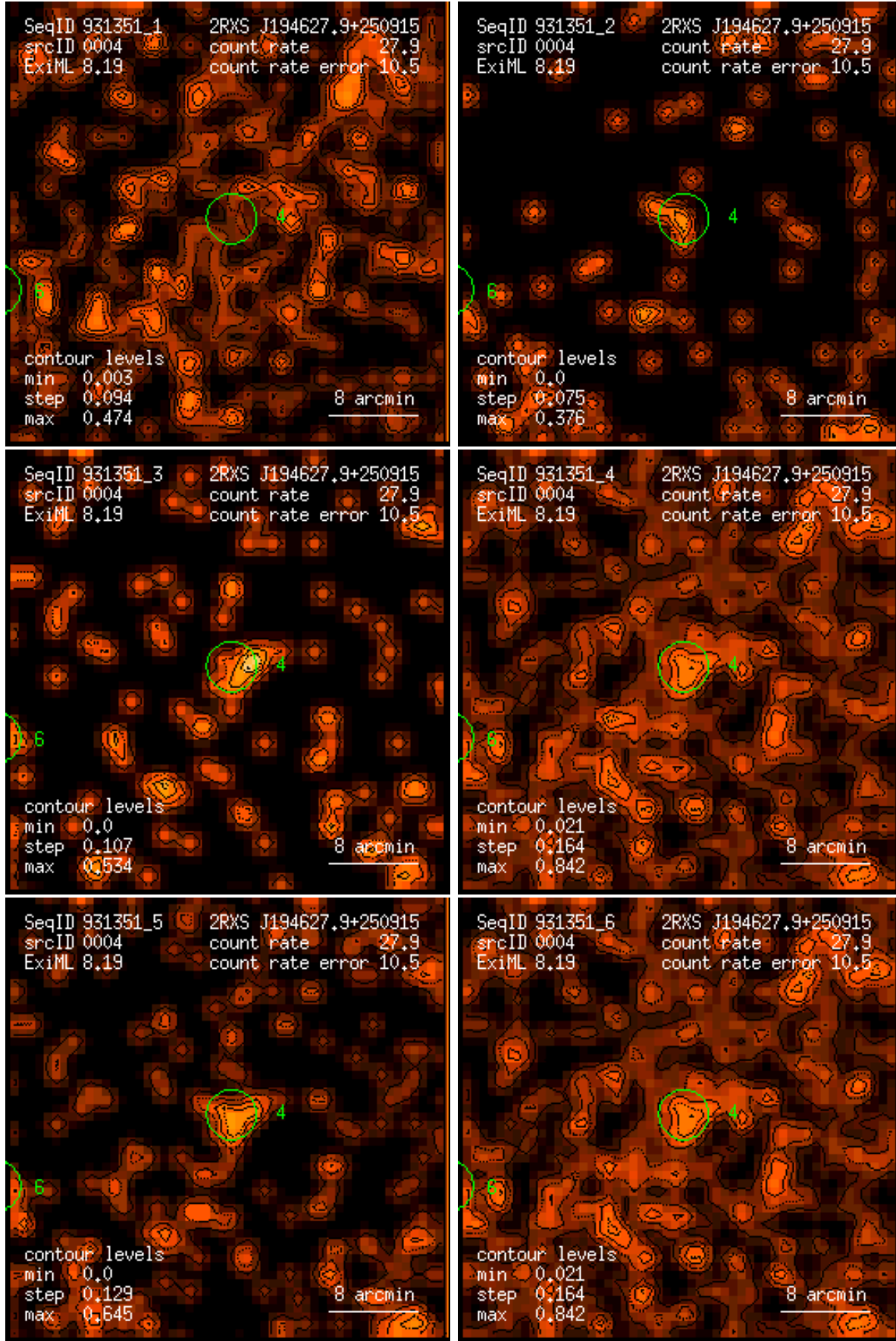
Figure 4: RASS 931351: detection 0004: band rate images, Gaussian filter: (1) PSPC channels 11 – 41, (2) 52 – 90, (3) 91 – 201, (4) 11 – 235, (5) 52 – 201, (6) 11 – 201. Broad band rates in counts/ks. Band rate contour levels in counts/ks/arcmin 2 .
