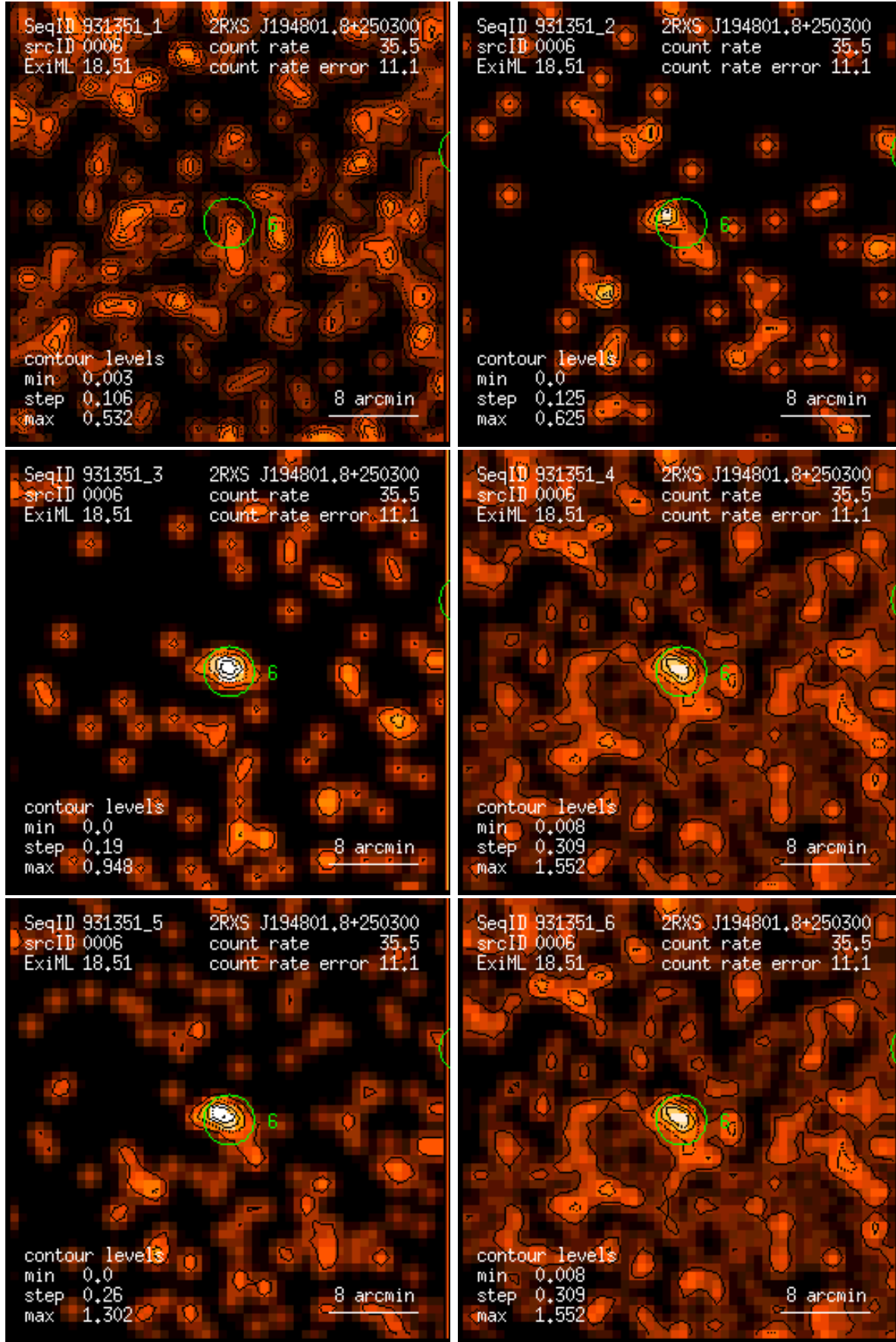
Figure 6: RASS 931351: detection 0006: band rate images, Gaussian filter: (1) PSPC channels 11 – 41, (2) 52 – 90, (3) 91 – 201, (4) 11 – 235, (5) 52 – 201, (6) 11 – 201. Broad band rates in counts/ks. Band rate contour levels in counts/ks/arcmin 2 .
