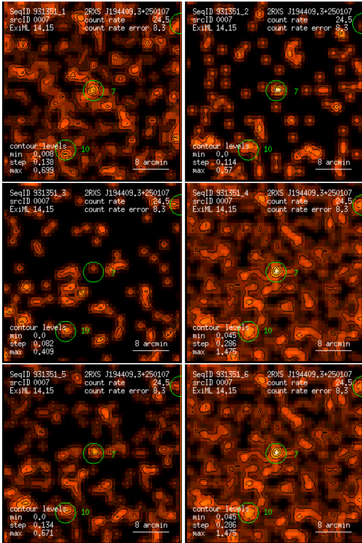
Figure 7: RASS 931351: detection 0007: band rate images, Gaussian filter: (1) PSPC channels 11 – 41, (2) 52 – 90, (3) 91 – 201, (4) 11 – 235, (5) 52 – 201, (6) 11 – 201. Broad band rates in counts/ks. Band rate contour levels in counts/ks/arcmin 2 .
