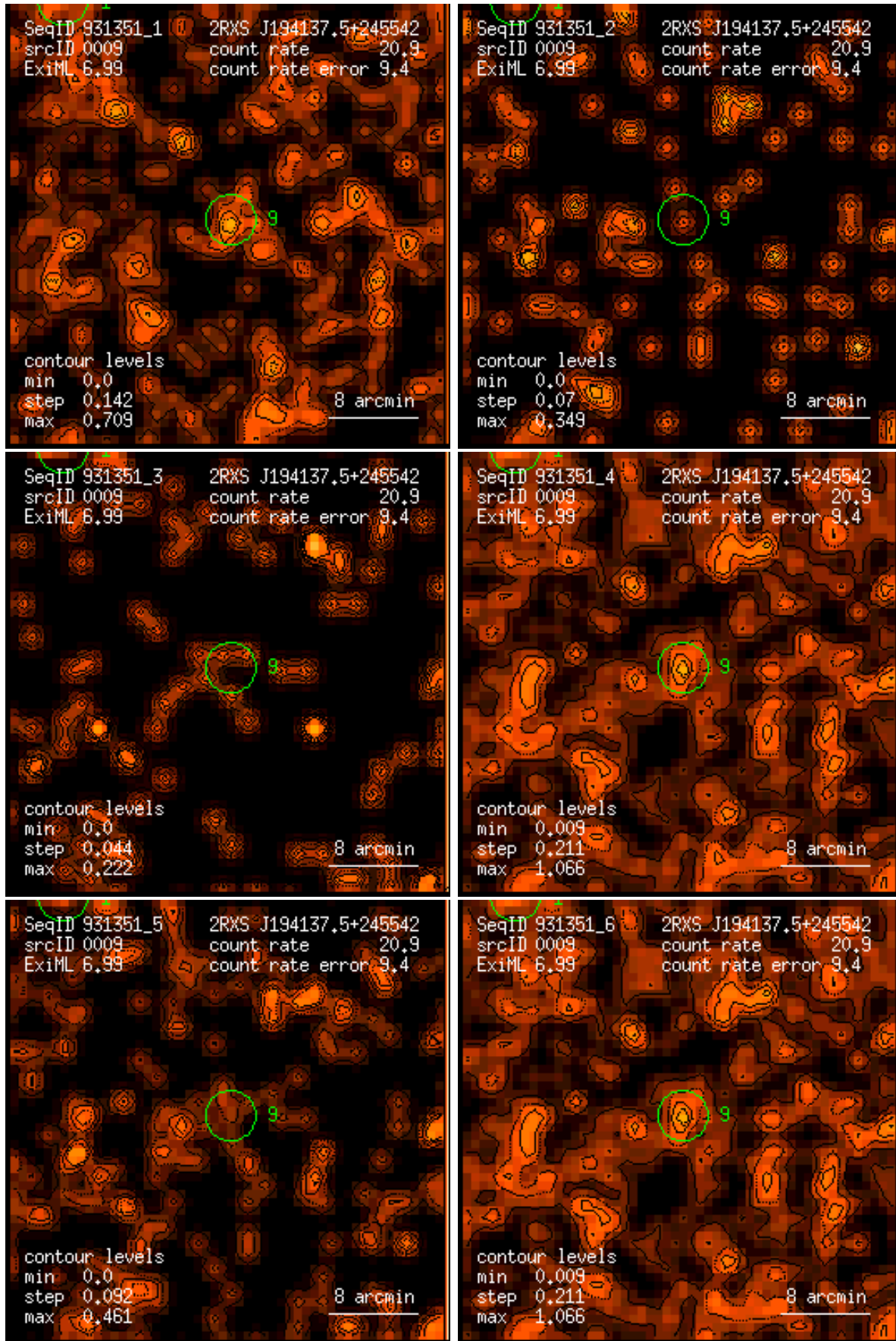
Figure 9: RASS 931351: detection 0009: band rate images, Gaussian filter: (1) PSPC channels 11 – 41, (2) 52 – 90, (3) 91 – 201, (4) 11 – 235, (5) 52 – 201, (6) 11 – 201. Broad band rates in counts/ks. Band rate contour levels in counts/ks/arcmin 2 .
