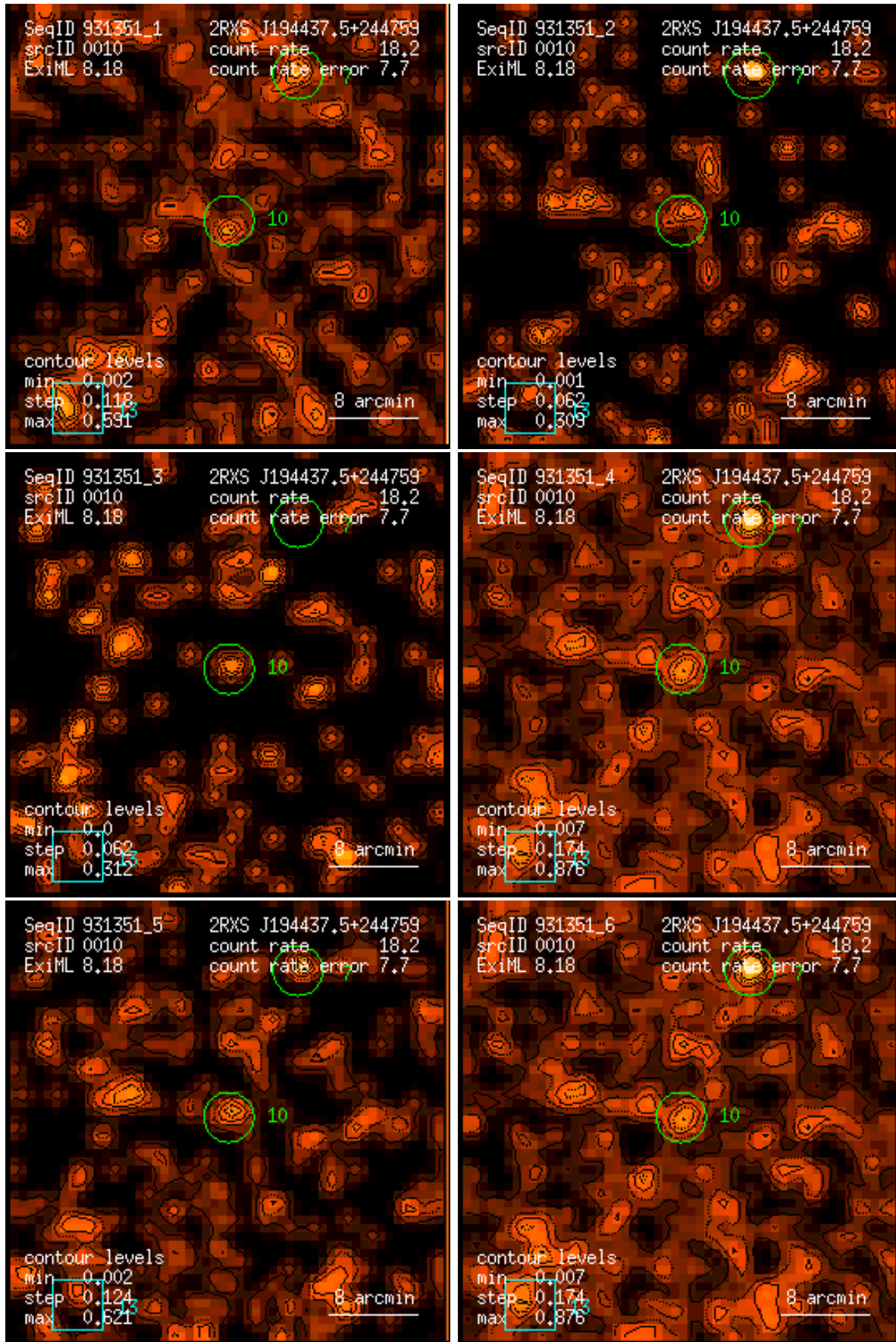
Figure 10: RASS 931351: detection 0010: band rate images, Gaussian filter: (1) PSPC channels 11 – 41, (2) 52 – 90, (3) 91 – 201, (4) 11 – 235, (5) 52 – 201, (6) 11 – 201. Broad band rates in counts/ks. Band rate contour levels in counts/ks/arcmin 2 .
