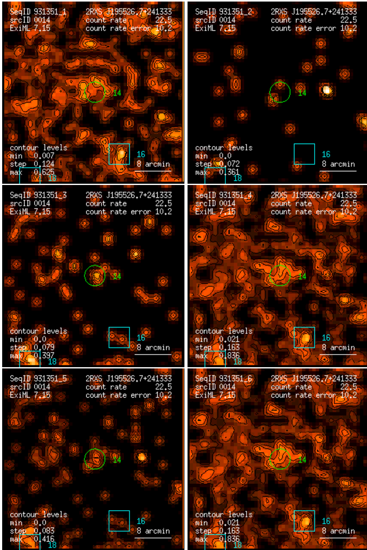
Figure 14: RASS 931351: detection 0014: band rate images, Gaussian filter: (1) PSPC channels 11 – 41, (2) 52 – 90, (3) 91 – 201, (4) 11 – 235, (5) 52 – 201, (6) 11 – 201. Broad band rates in counts/ks. Band rate contour levels in counts/ks/arcmin 2 .
