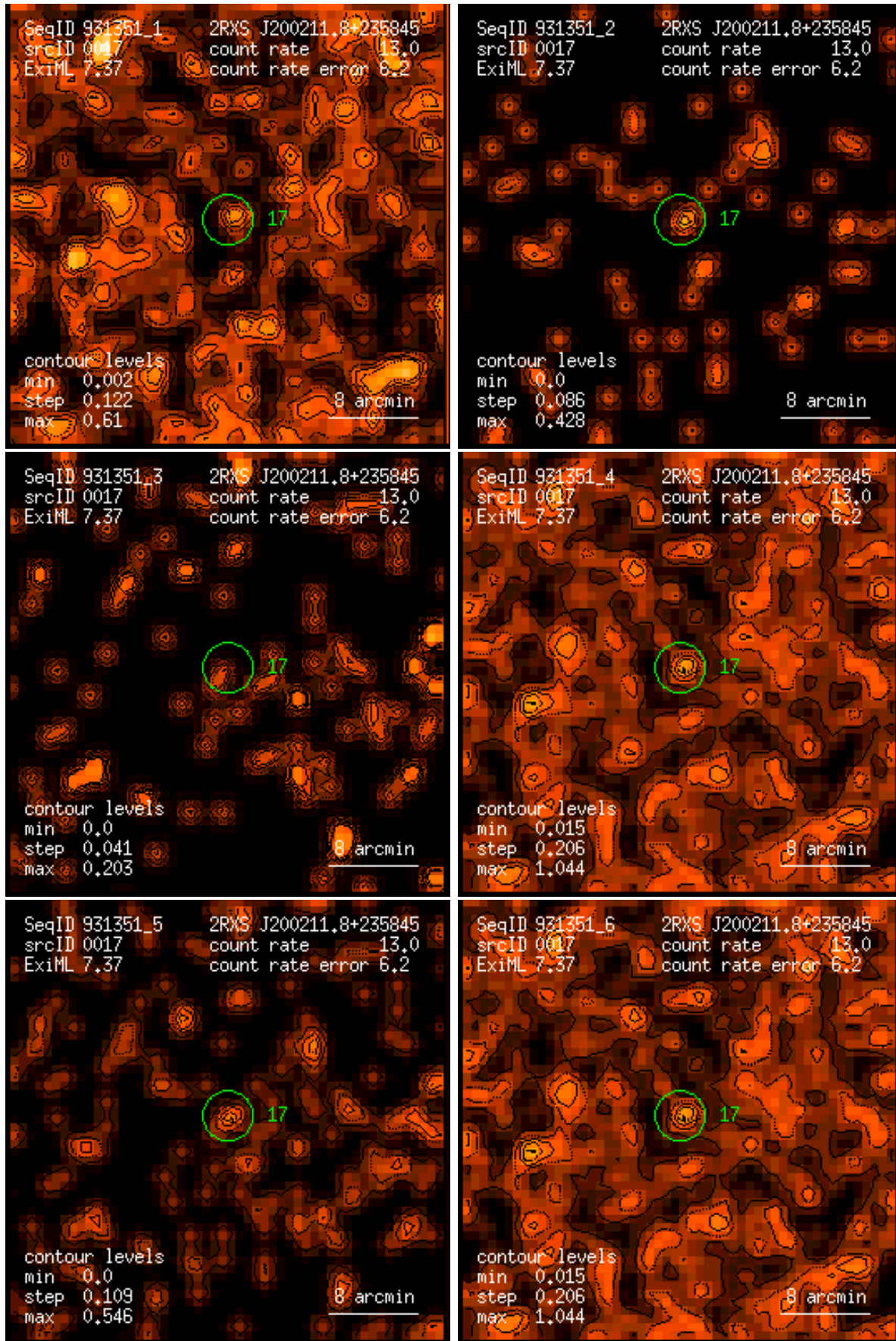
Figure 17: RASS 931351: detection 0017: band rate images, Gaussian filter: (1) PSPC channels 11 – 41, (2) 52 – 90, (3) 91 – 201, (4) 11 – 235, (5) 52 – 201, (6) 11 – 201. Broad band rates in counts/ks. Band rate contour levels in counts/ks/arcmin 2 .
