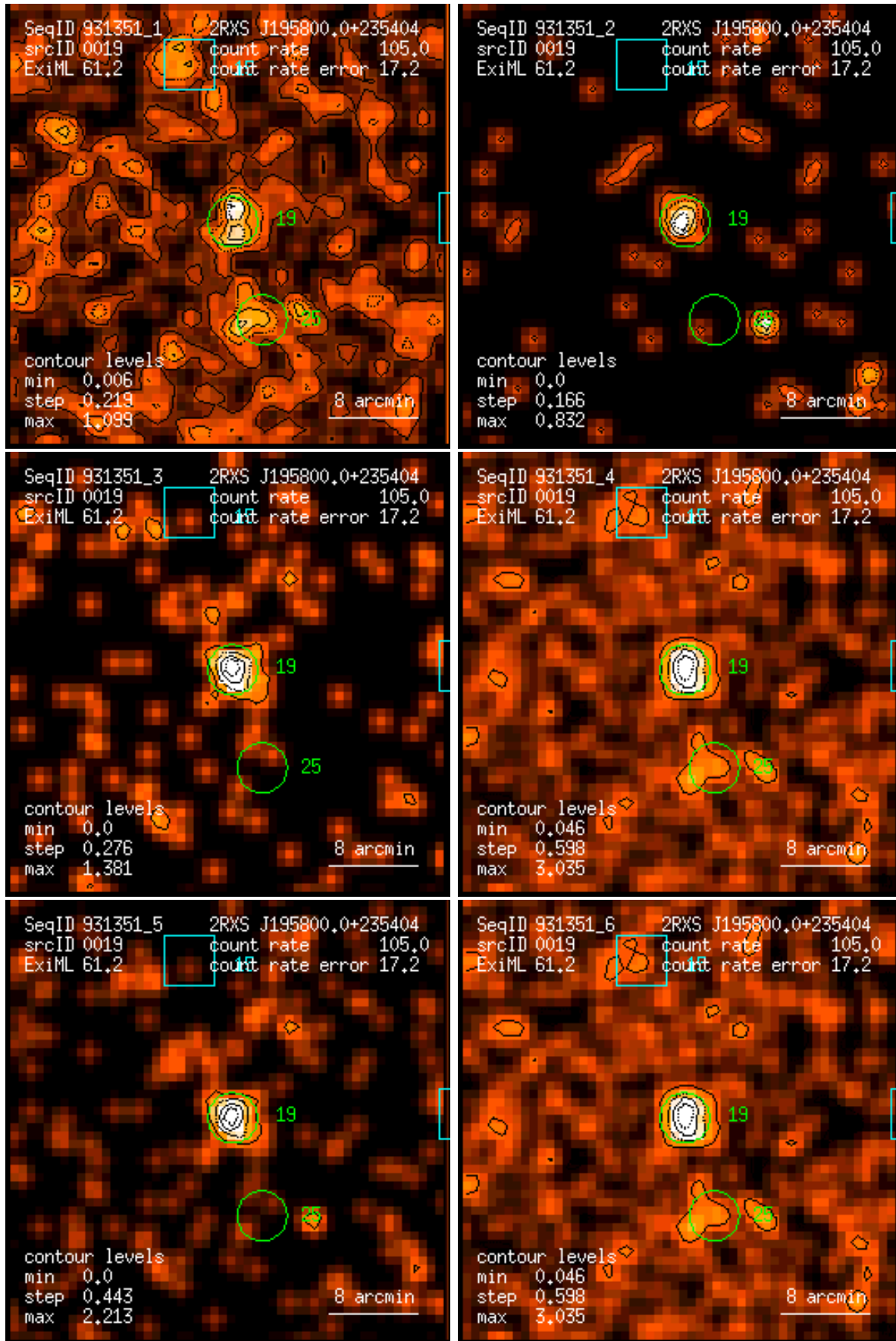
Figure 19: RASS 931351: detection 0019: band rate images, Gaussian filter: (1) PSPC channels 11 – 41, (2) 52 – 90, (3) 91 – 201, (4) 11 – 235, (5) 52 – 201, (6) 11 – 201. Broad band rates in counts/ks. Band rate contour levels in counts/ks/arcmin 2 .
