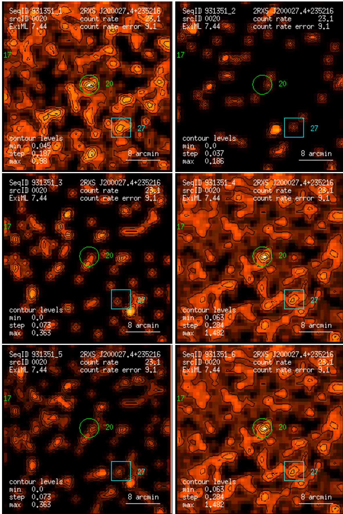
Figure 20: RASS 931351: detection 0020: band rate images, Gaussian filter: (1) PSPC channels 11 – 41, (2) 52 – 90, (3) 91 – 201, (4) 11 – 235, (5) 52 – 201, (6) 11 – 201. Broad band rates in counts/ks. Band rate contour levels in counts/ks/arcmin 2 .
