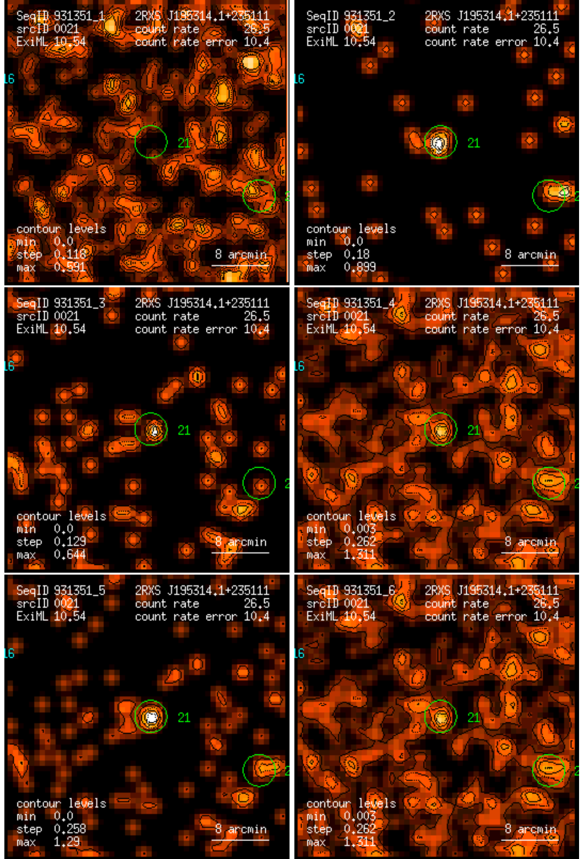
Figure 21: RASS 931351: detection 0021: band rate images, Gaussian filter: (1) PSPC channels 11 – 41, (2) 52 – 90, (3) 91 – 201, (4) 11 – 235, (5) 52 – 201, (6) 11 – 201. Broad band rates in counts/ks. Band rate contour levels in counts/ks/arcmin 2 .
