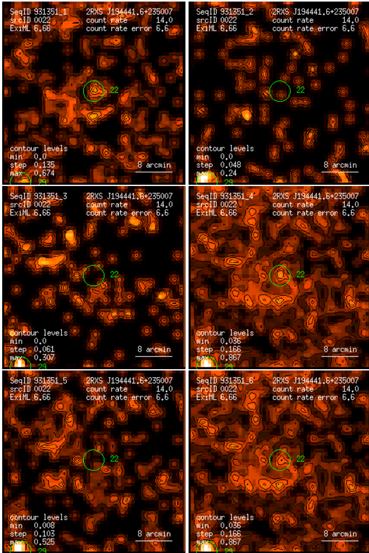
Figure 22: RASS 931351: detection 0022: band rate images, Gaussian filter: (1) PSPC channels 11 – 41, (2) 52 – 90, (3) 91 – 201, (4) 11 – 235, (5) 52 – 201, (6) 11 – 201. Broad band rates in counts/ks. Band rate contour levels in counts/ks/arcmin 2 .
